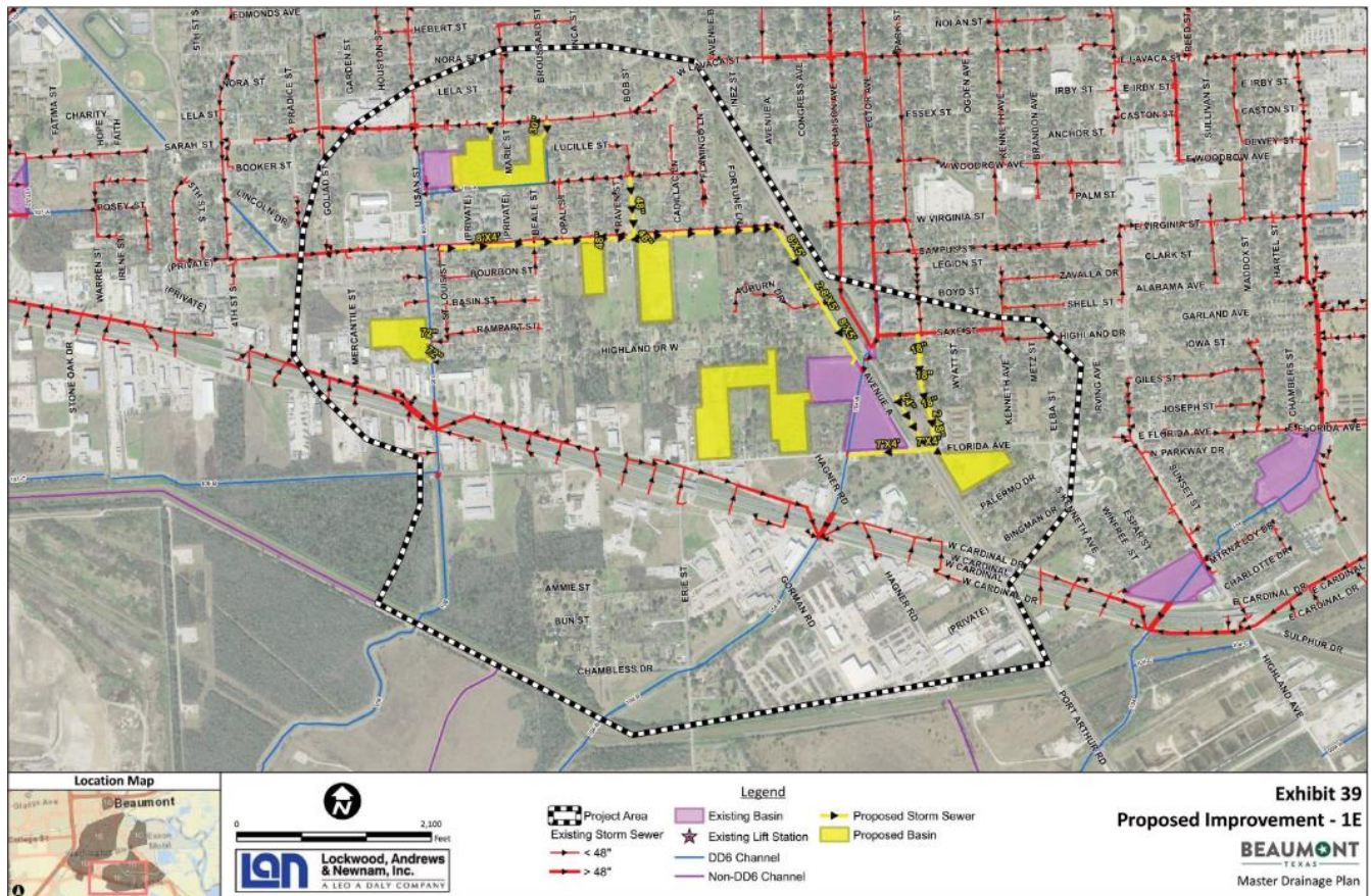
FIGURE 5-31: VIRGINIA STREET DETENTION PROJECT EXTENTS
