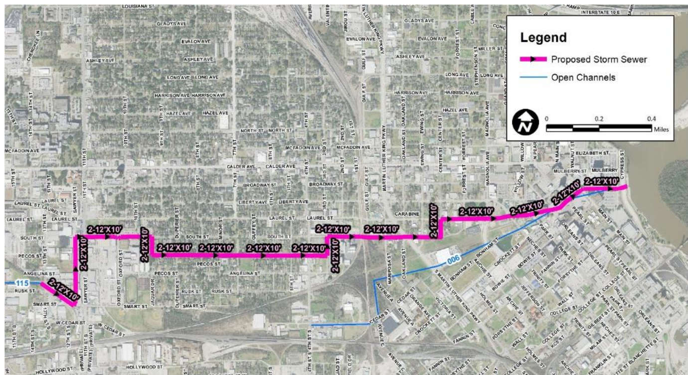
FIGURE 5-28: TEVIS DIVERSION PROJECT EXTENTS
