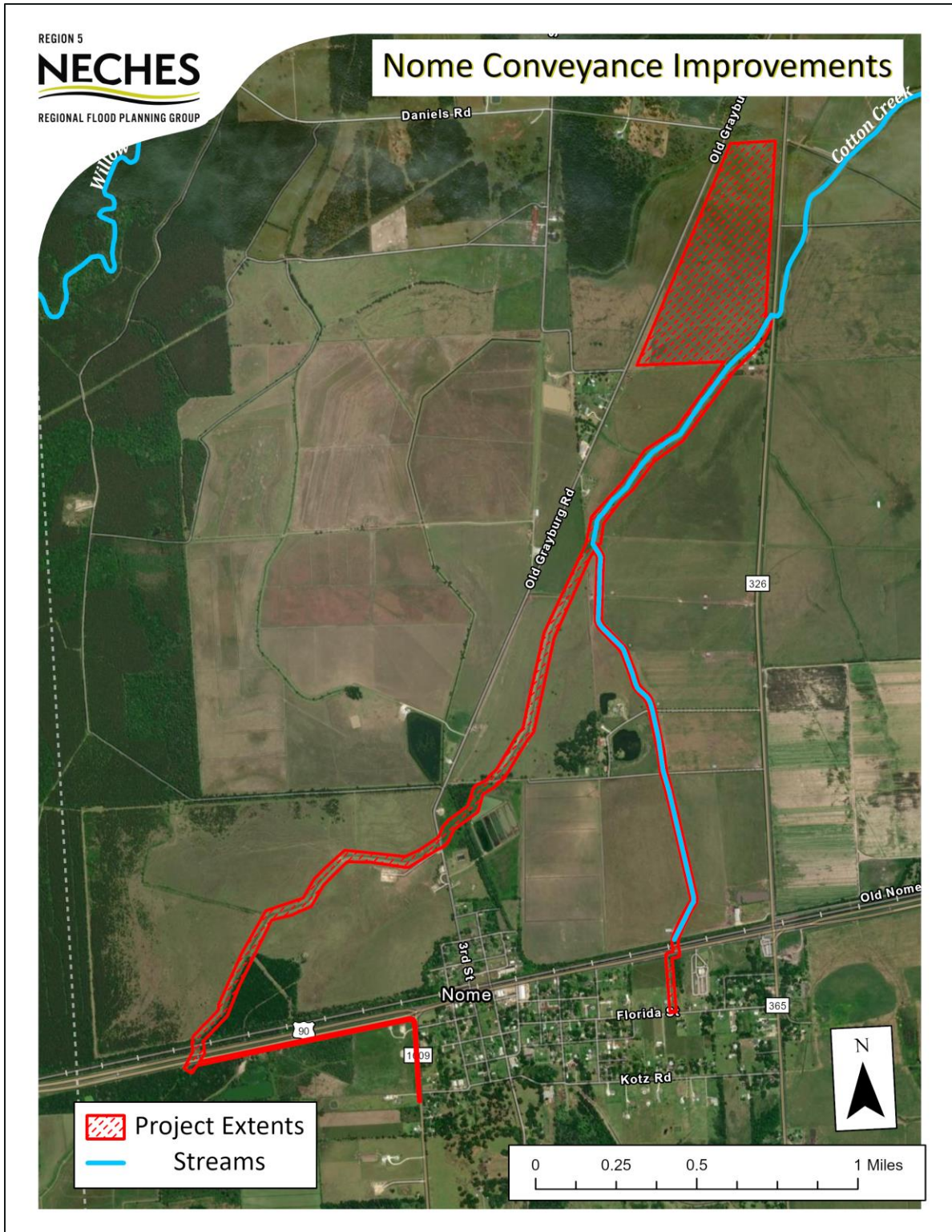
FIGURE 5-14: NOME CONVEYANCE IMPROVEMENTS PROJECT EXTENTS
