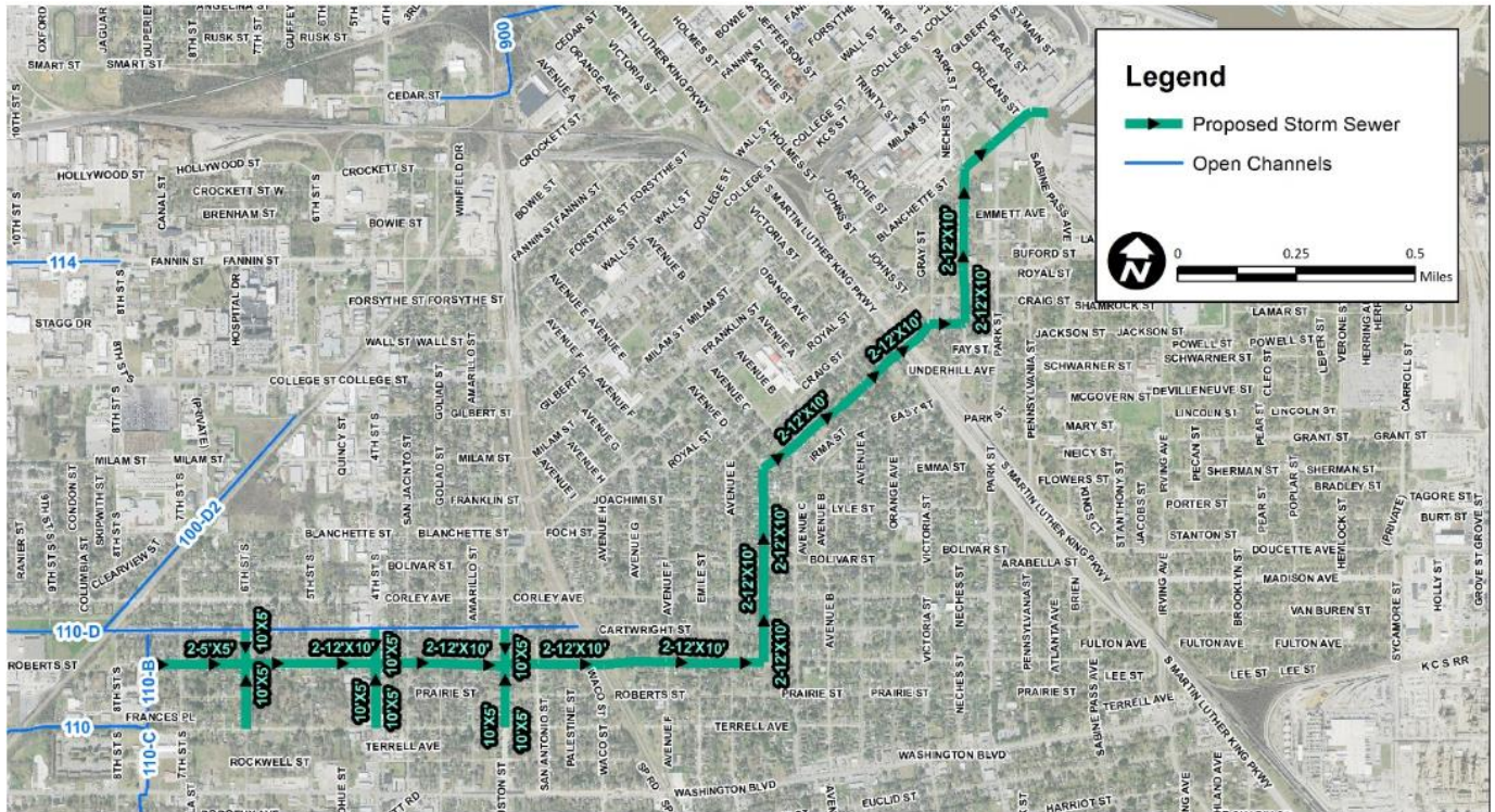
FIGURE 5-29: BLANCHETTE DIVERSION PROJECT EXTENTS
