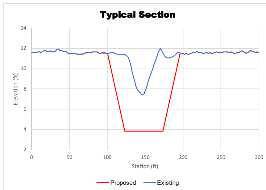
FIGURE 5-23: TYRRELL PARK IMPROVEMENTS TYPICAL SECTION
