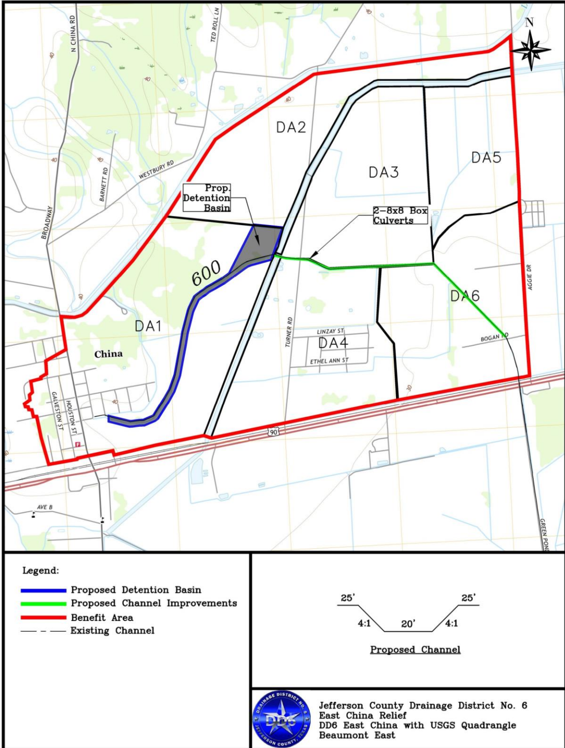
FIGURE 5-34: EAST CHINA RELIEF PROJECT EXTENTS
