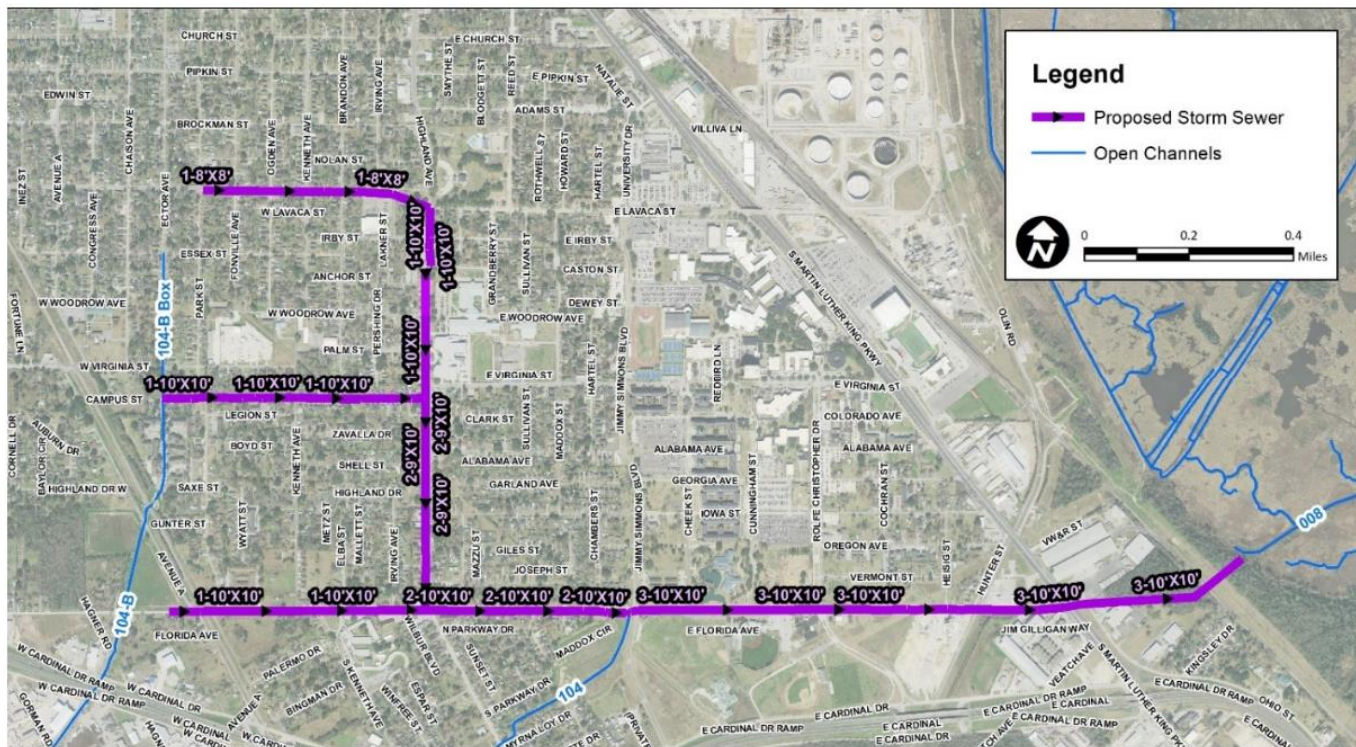
FIGURE 5-27: SOUTH PARK DIVERSION PROJECT EXTENTS
