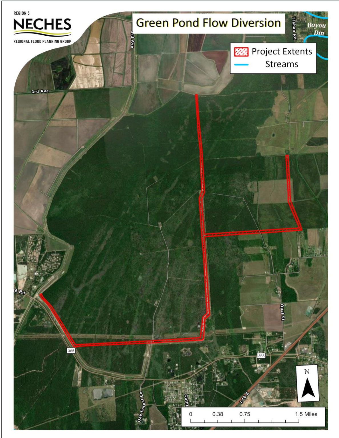
FIGURE 5-25: GREEN POND FLOW DIVERSION PROJECT EXTENTS
