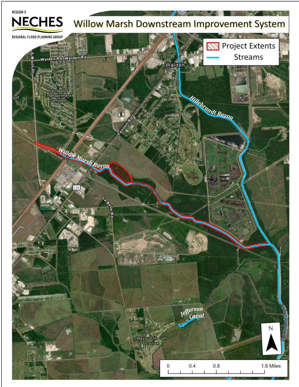
FIGURE 5-22: WILLOW MARSH DOWNSTREAM IMPROVEMENT SYSTEM PROJECT EXTENTS
