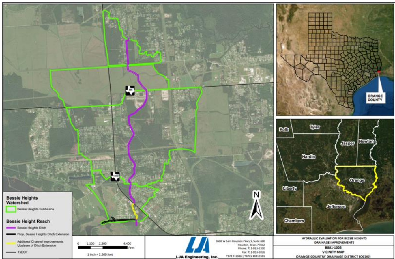
FIGURE 5-4: BESSIE HEIGHTS DRAINAGE DITCH EXTENSION PROJECT EXTENTS
