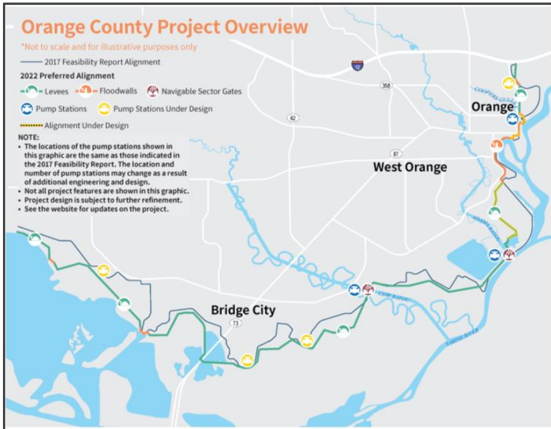
FIGURE 5-6: ORANGE COUNTY COASTAL STORM RISK MANAGEMENT PROJECT EXTENTS
