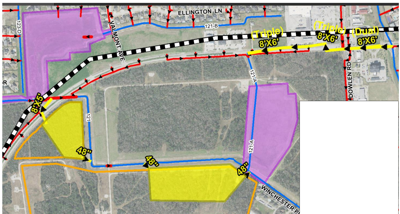
FIGURE 5-32: DELAWARE HILCORP DETENTION PROJECT EXTENTS
