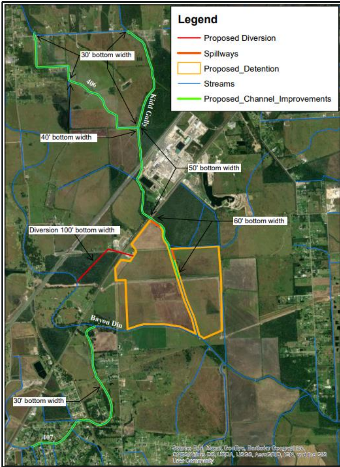
FIGURE 5-3: BAYOU DIN DETENTION BASIN PROJECT EXTENTS
