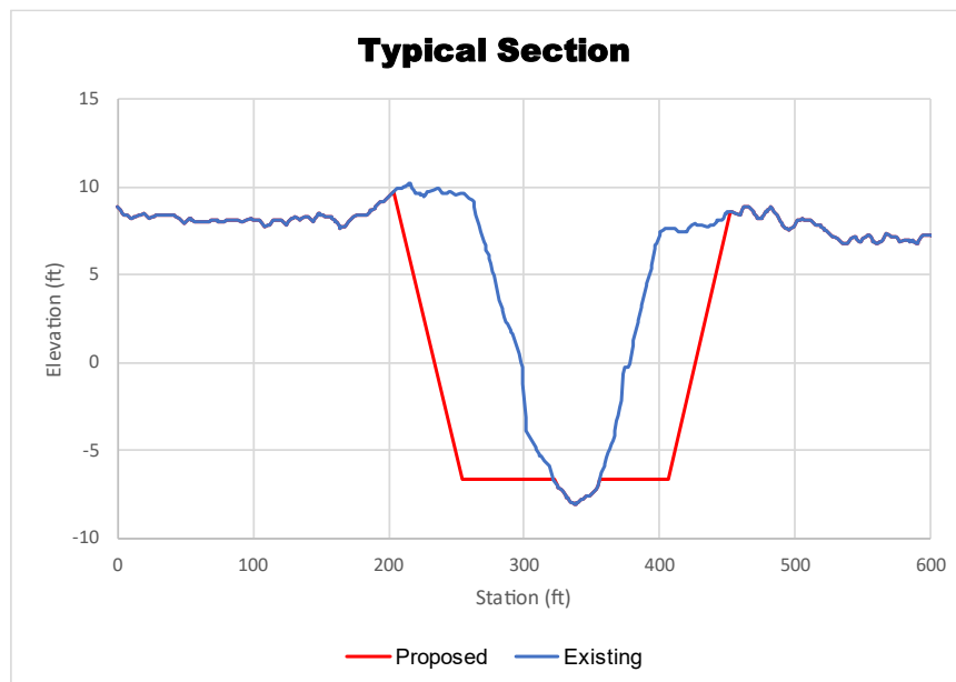
FIGURE 5-21: WILLOW MARSH DOWNSTREAM IMPROVEMENT SYSTEM TYPICAL SECTION
