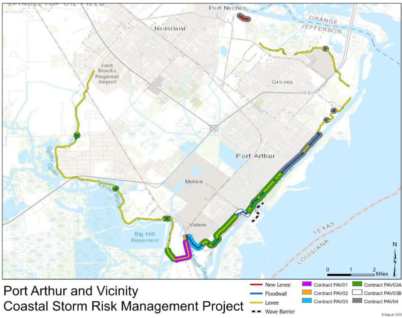
FIGURE 5-5: PORT ARTHUR AND VICINITY COASTAL STORM RISK MANAGEMENT PROJECT EXTENTS
