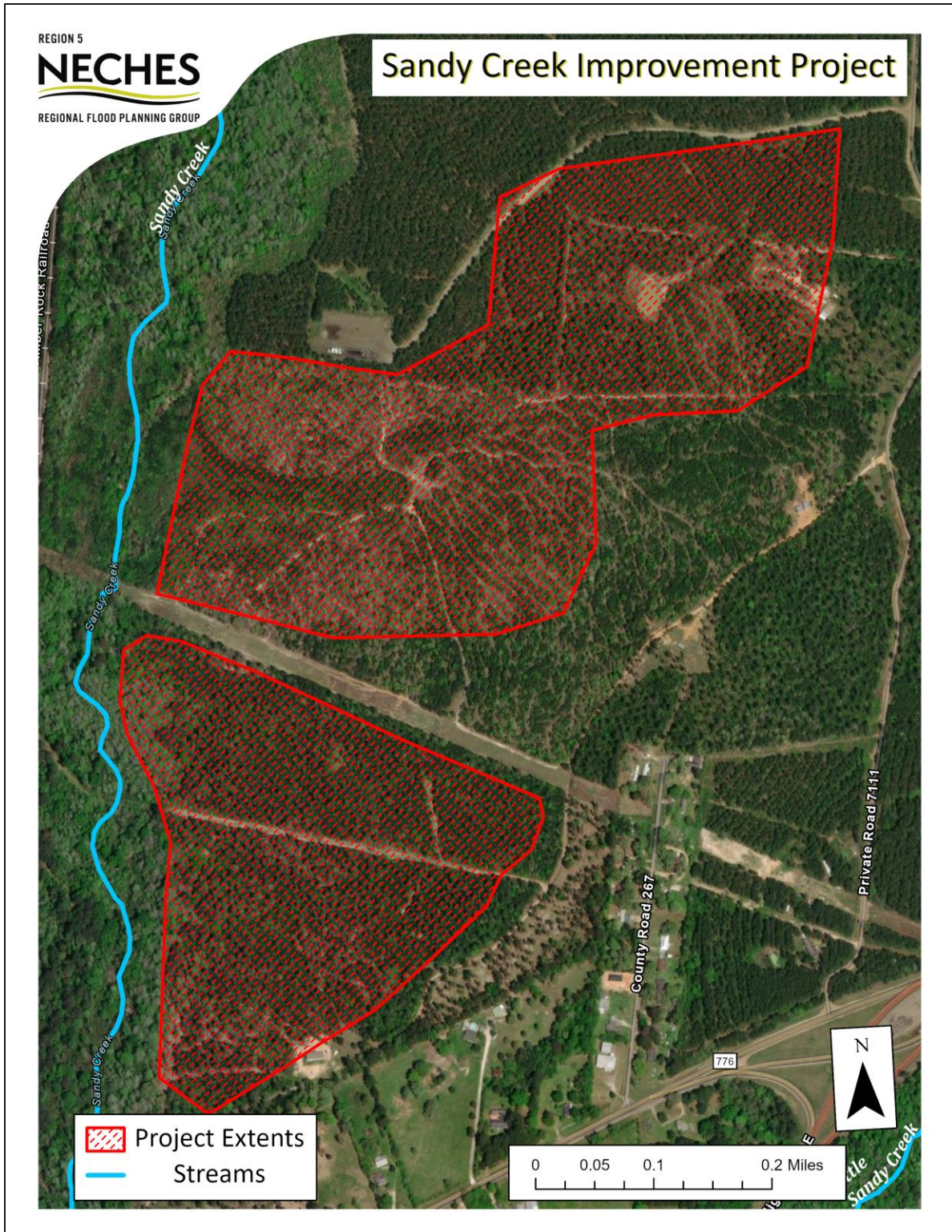
FIGURE 5-8: SANDY CREEK IMPROVEMENT PROJECT EXTENTS
