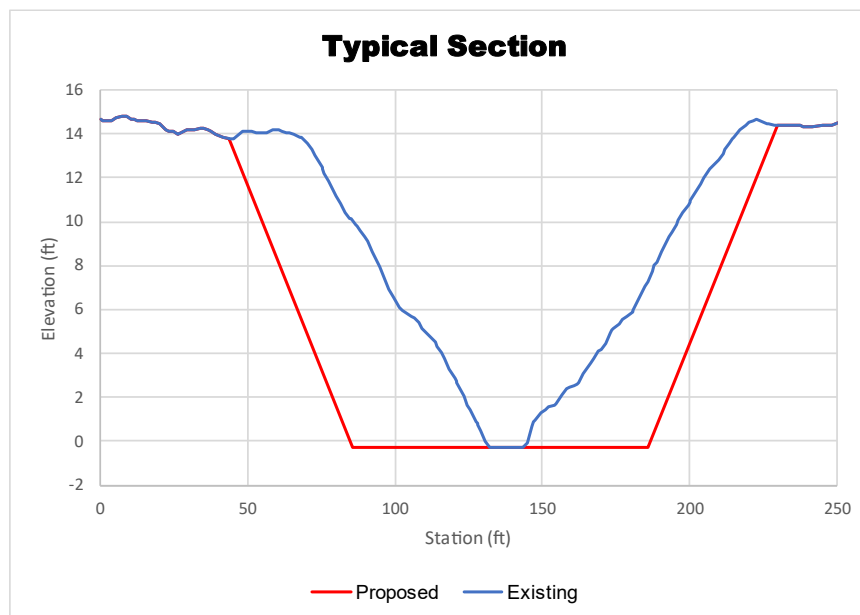
FIGURE 5-19: WILLOW MARSH MAIN IMPROVEMENT SYSTEM TYPICAL SECTION
