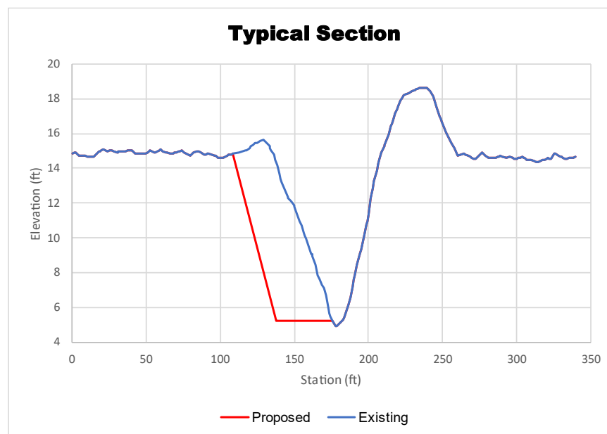
FIGURE 5-15: PEVITOT GULLY IMPROVEMENT SYSTEM TYPICAL SECTION
