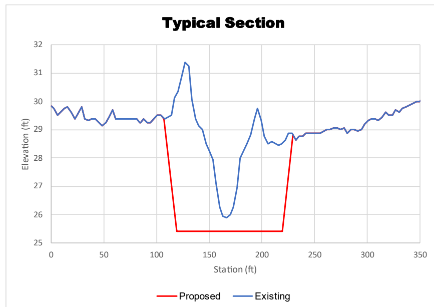
FIGURE 5-9: SOUR LAKE CHANNEL IMPROVEMENTS TYPICAL SECTION
