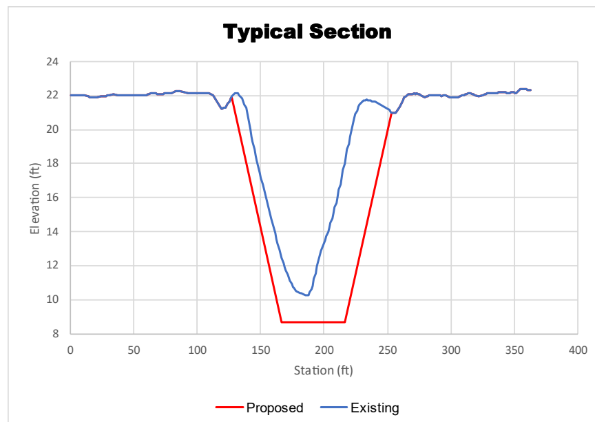
FIGURE 5-11: ROSEDALE IMPROVEMENT SYSTEM TYPICAL SECTION
