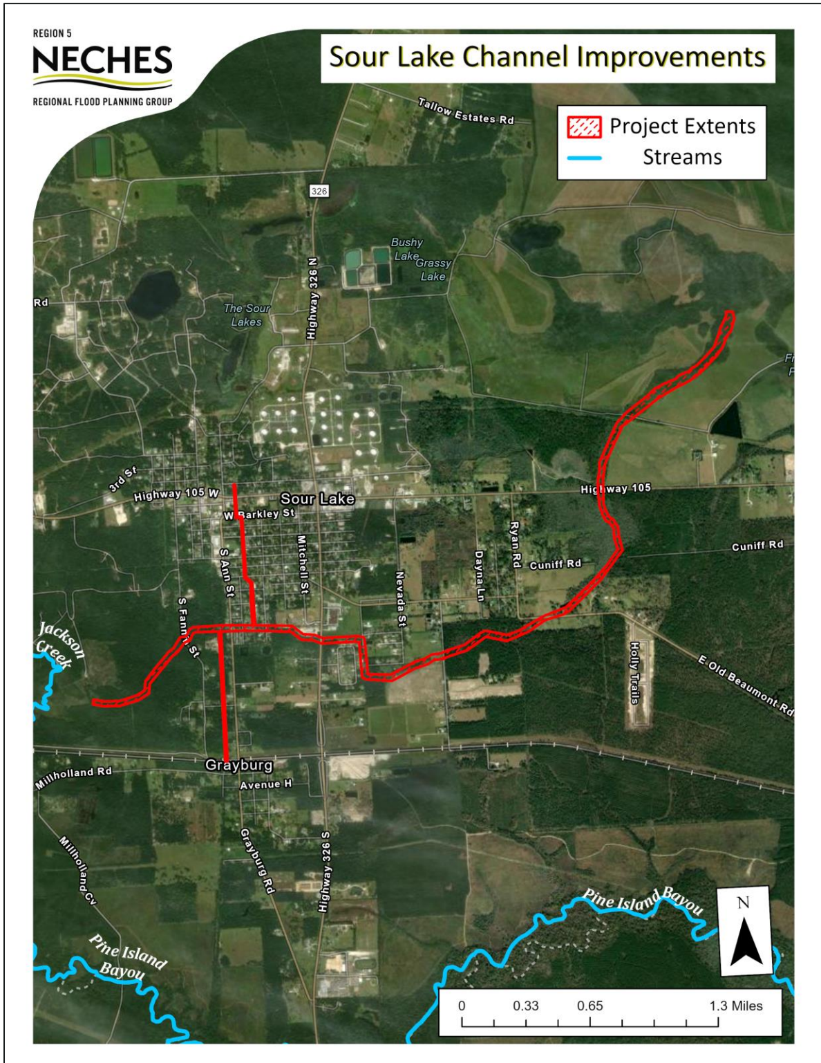
FIGURE 5-10: SOUR LAKE CHANNEL IMPROVEMENTS PROJECT EXTENTS
