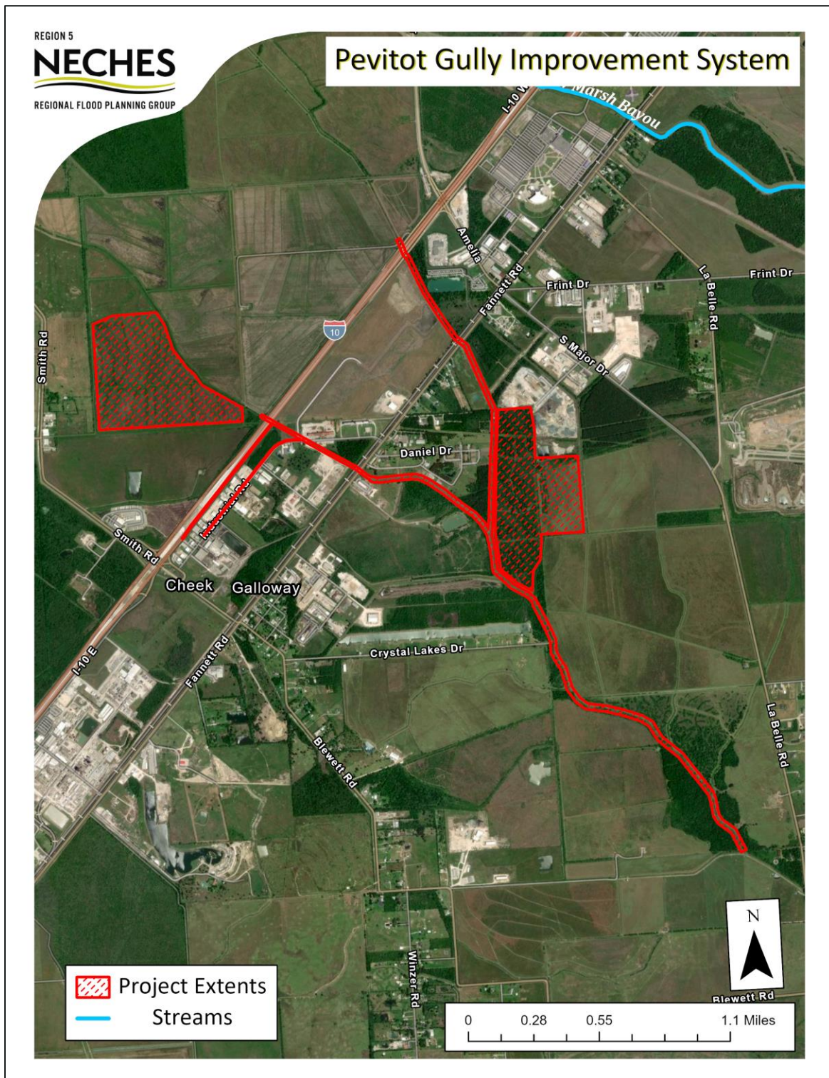
FIGURE 5-16: PEVITOT GULLY IMPROVEMENT SYSTEM PROJECT EXTENTS
