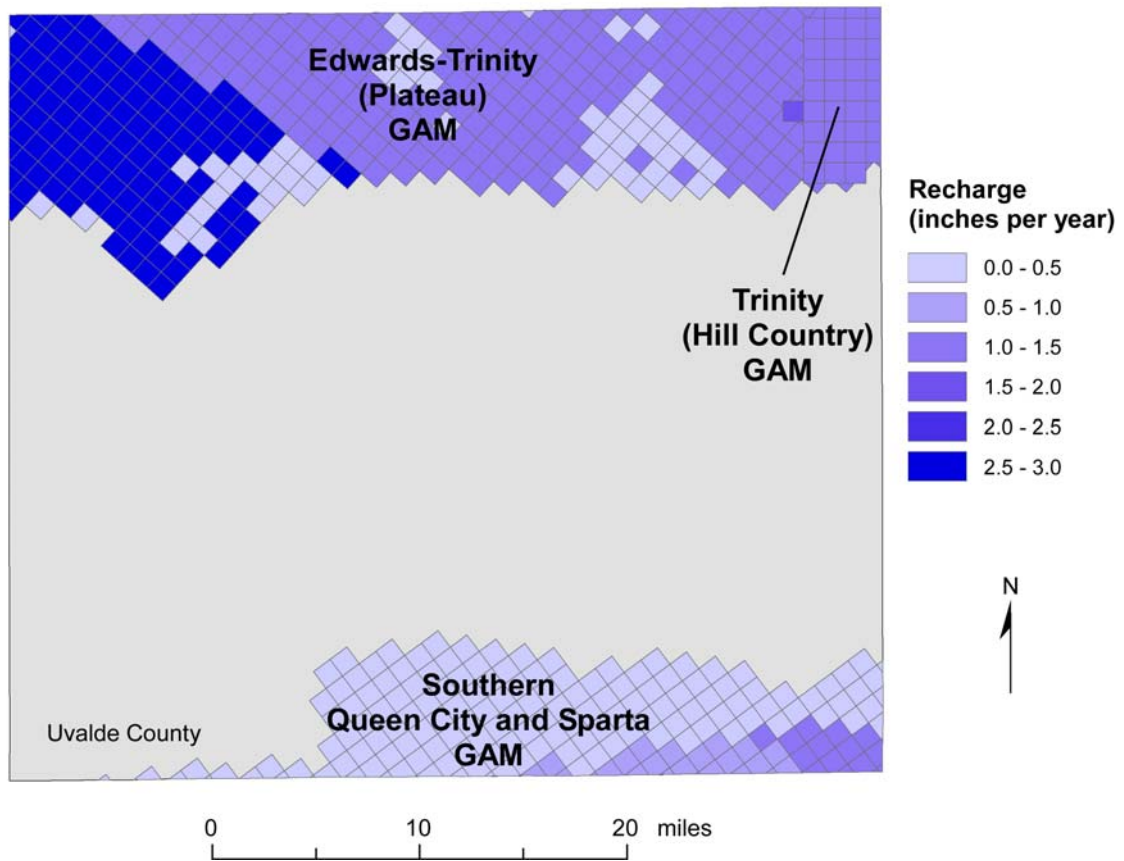
Figure 1. Distribution of average annual recharge rates for active model cells of the Trinity (Hill Country) GAM, Edwards-Trinity (Plateau) GAM, and southern part of the Carrizo-Wilcox aquifer contained within the Queen City and Sparta aquifer GAM within Uvalde County.
