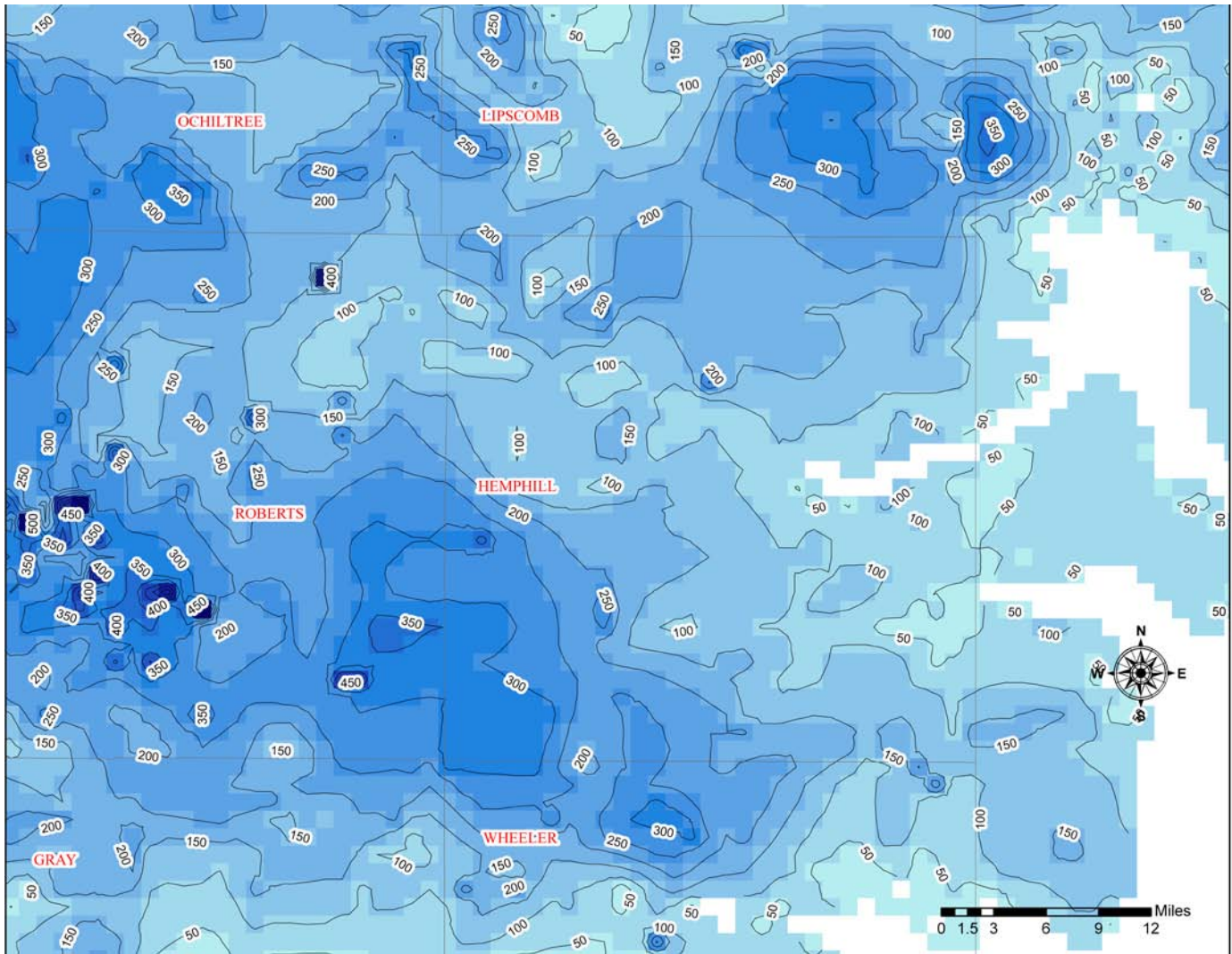
Figure 5: 2020 saturated thickness on the eastern side of the northern portion of the Ogallala Aquifer. White cells are inactive and/or outside the boundary of the model.
