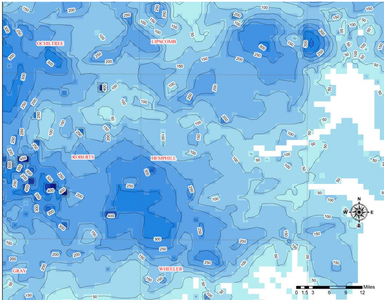
Figure 6: 2030 saturated thickness on the eastern side of the northern portion of the Ogallala Aquifer. White cells are inactive and/or outside the boundary of the model.
