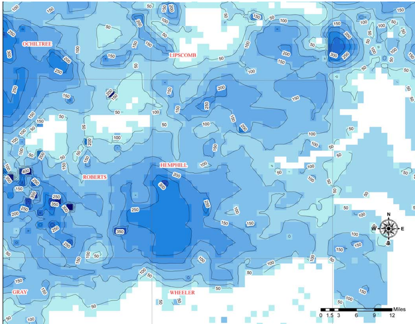
Figure 9: 2060 saturated thickness on the eastern side of the northern portion of the Ogallala Aquifer. White cells are inactive and/or outside the boundary of the model.
