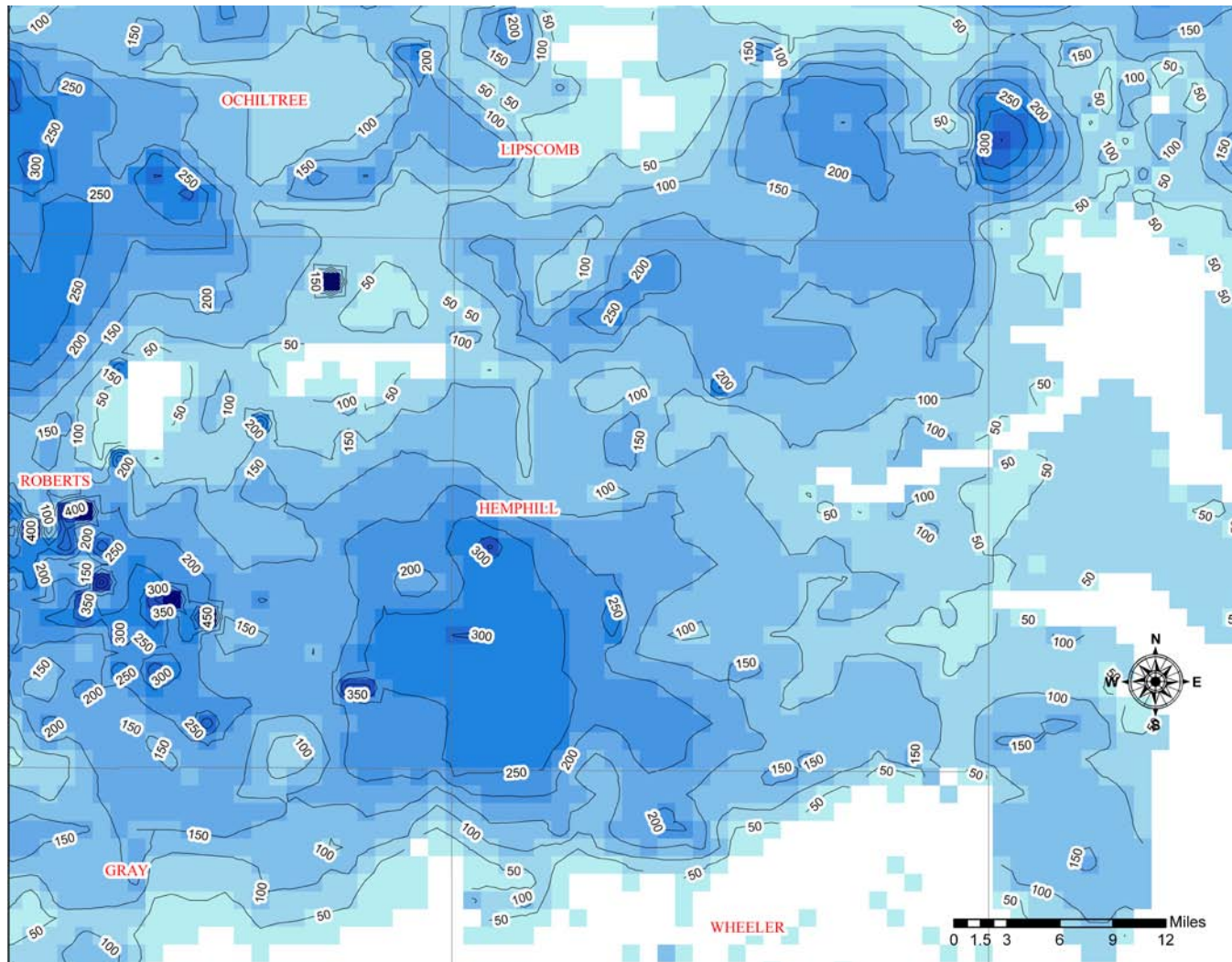
Figure 8: 2050 saturated thickness on the eastern side of the northern portion of the Ogallala Aquifer. White cells are inactive and/or outside the boundary of the model.
