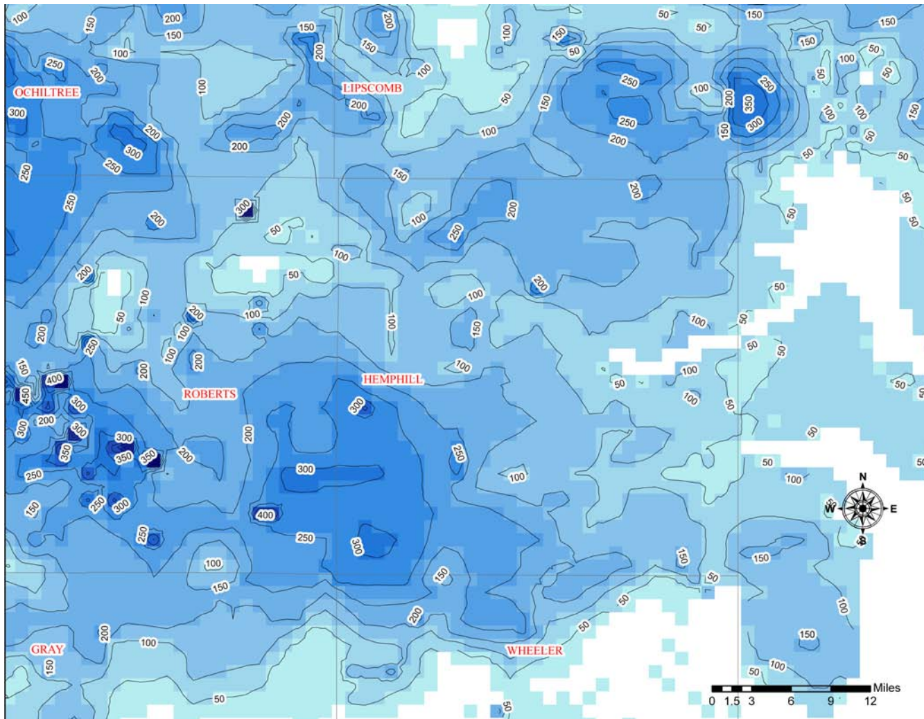
Figure 7: 2040 saturated thickness on the eastern side of the northern portion of the Ogallala Aquifer. White cells are inactive and/or outside the boundary of the model.
