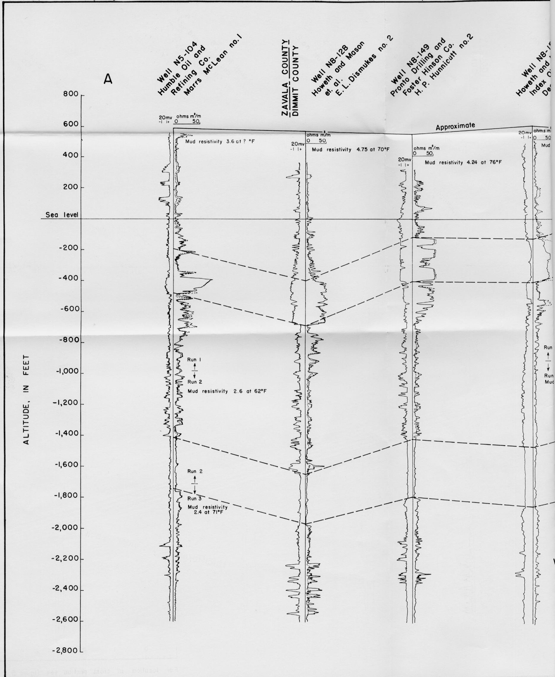
GEOLOGIC CROSS SECTION ALONG
