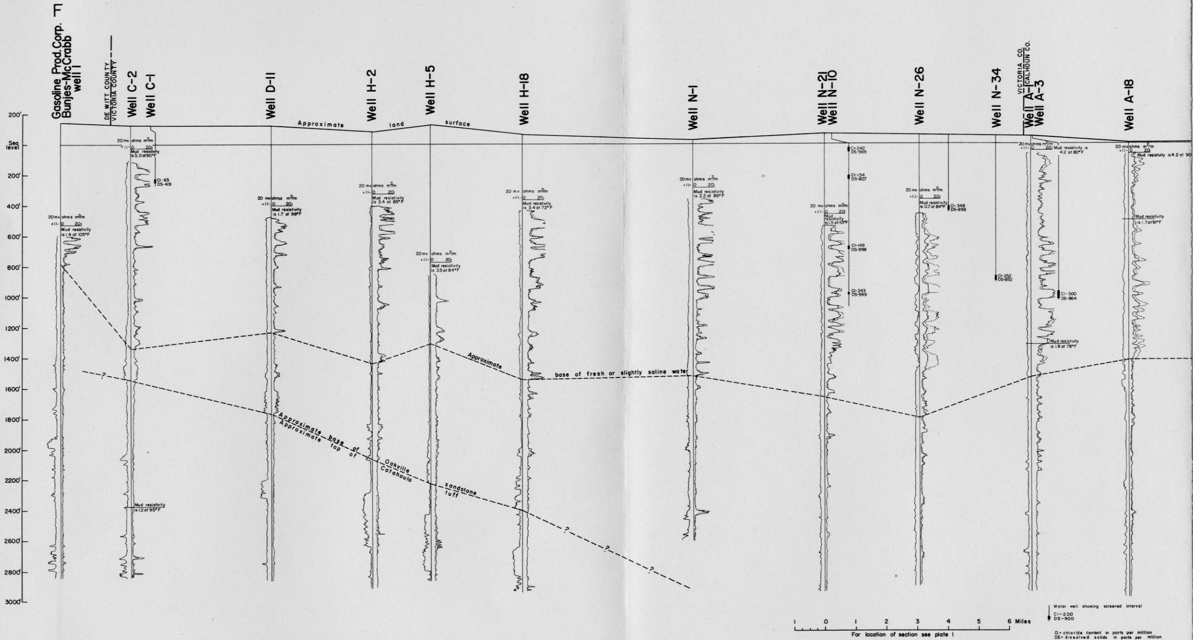
CROSS SECTION F-F', VICTORIA AND CALHOUN COUNTIES, TEXAS
