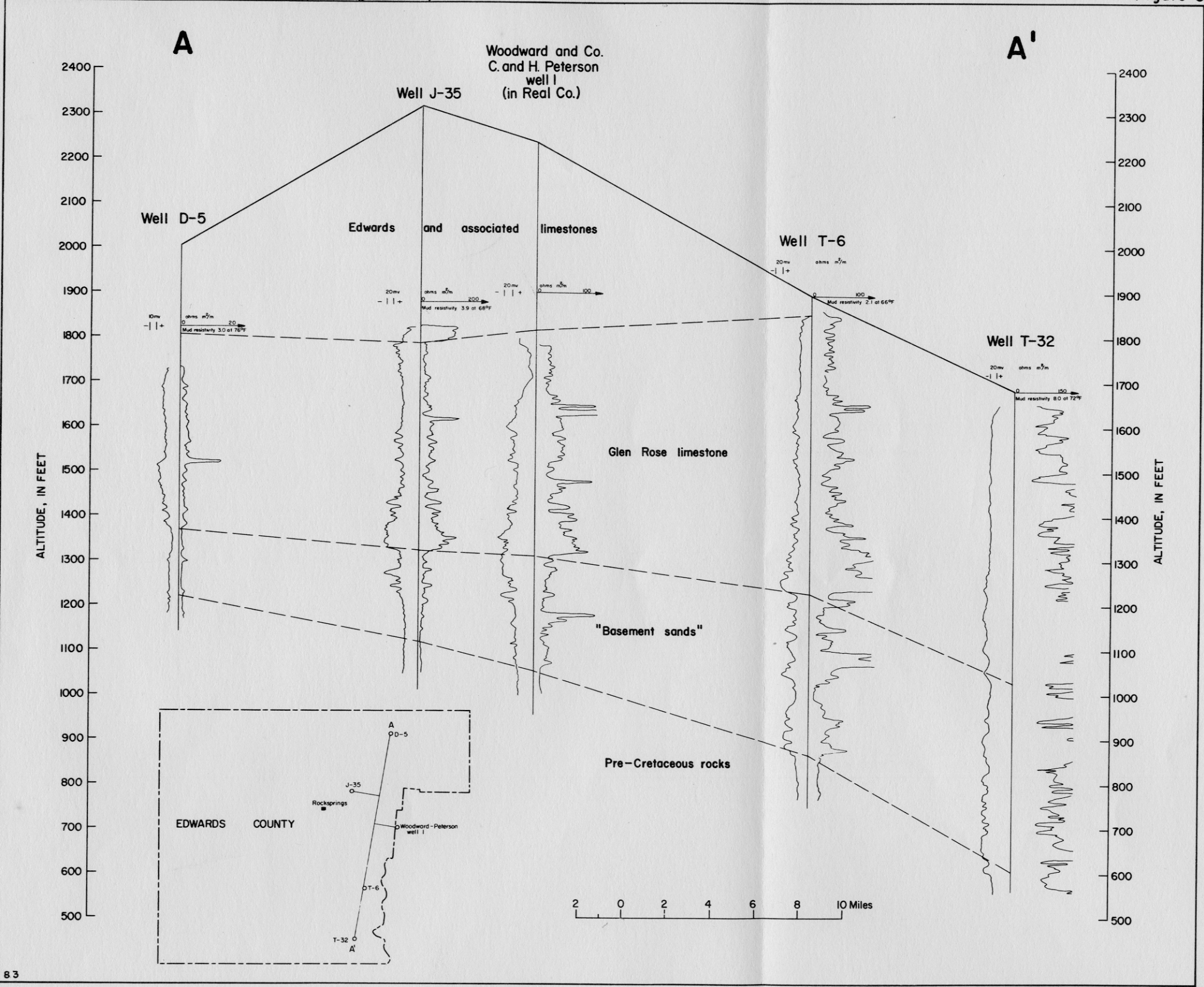
FIGURE 5. - Geologic section A-A', Edwards County
