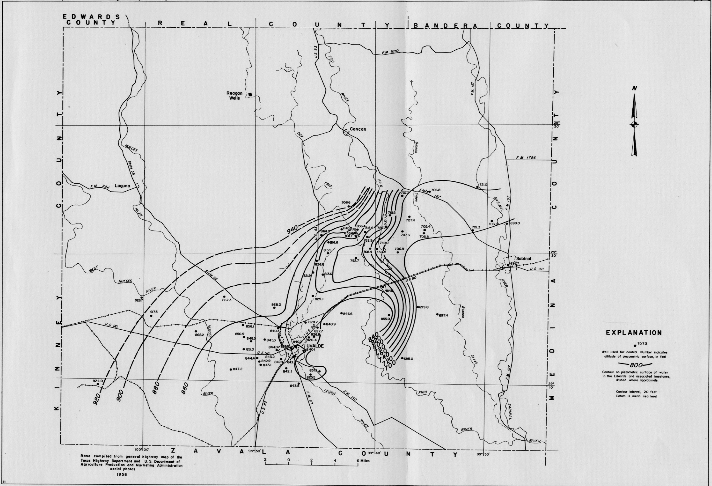
FIGURE 8.—Map of Uvalde County, showing contours on piezometric surface of water in the Edwards and associated limestones, December 1957
