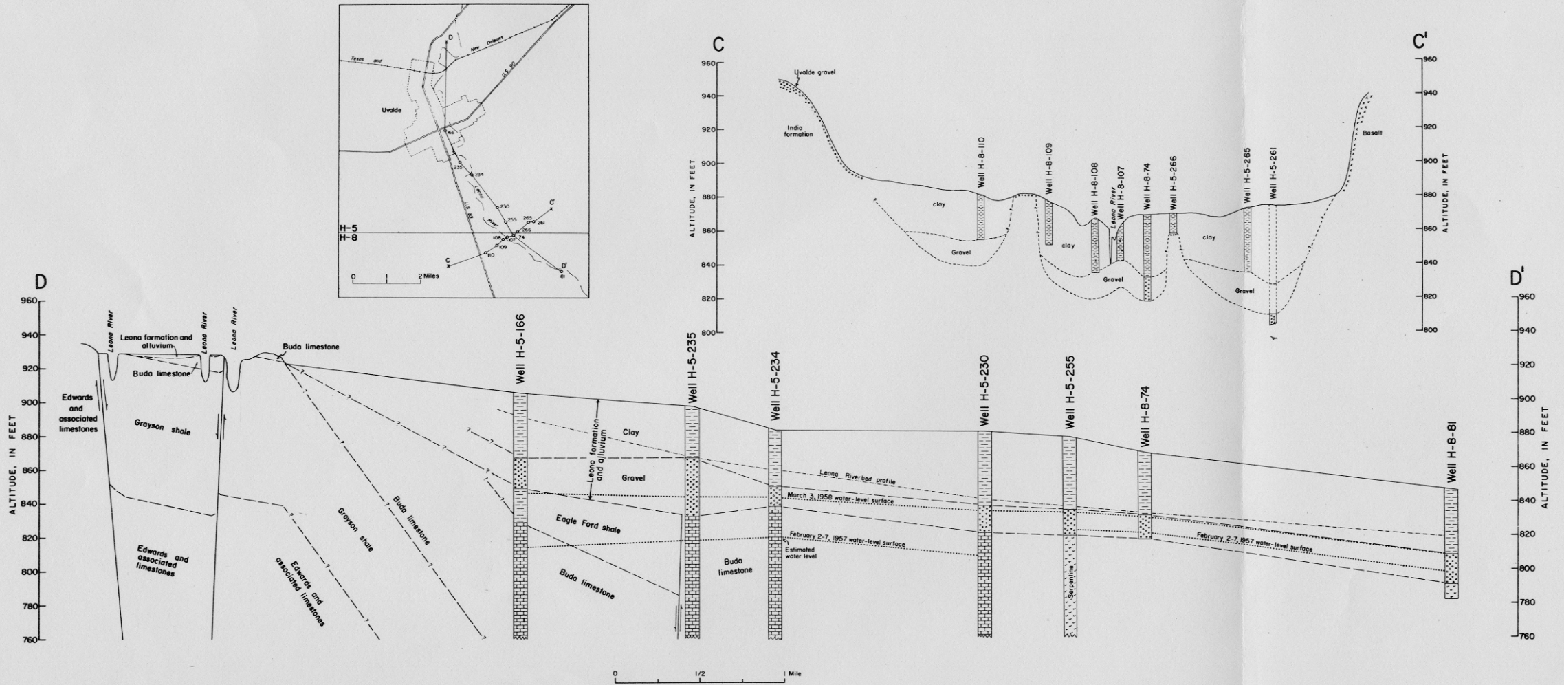
GEOLOGIC SECTIONS IN THE LEONA RIVER VALLEY, UVALDE COUNTY
