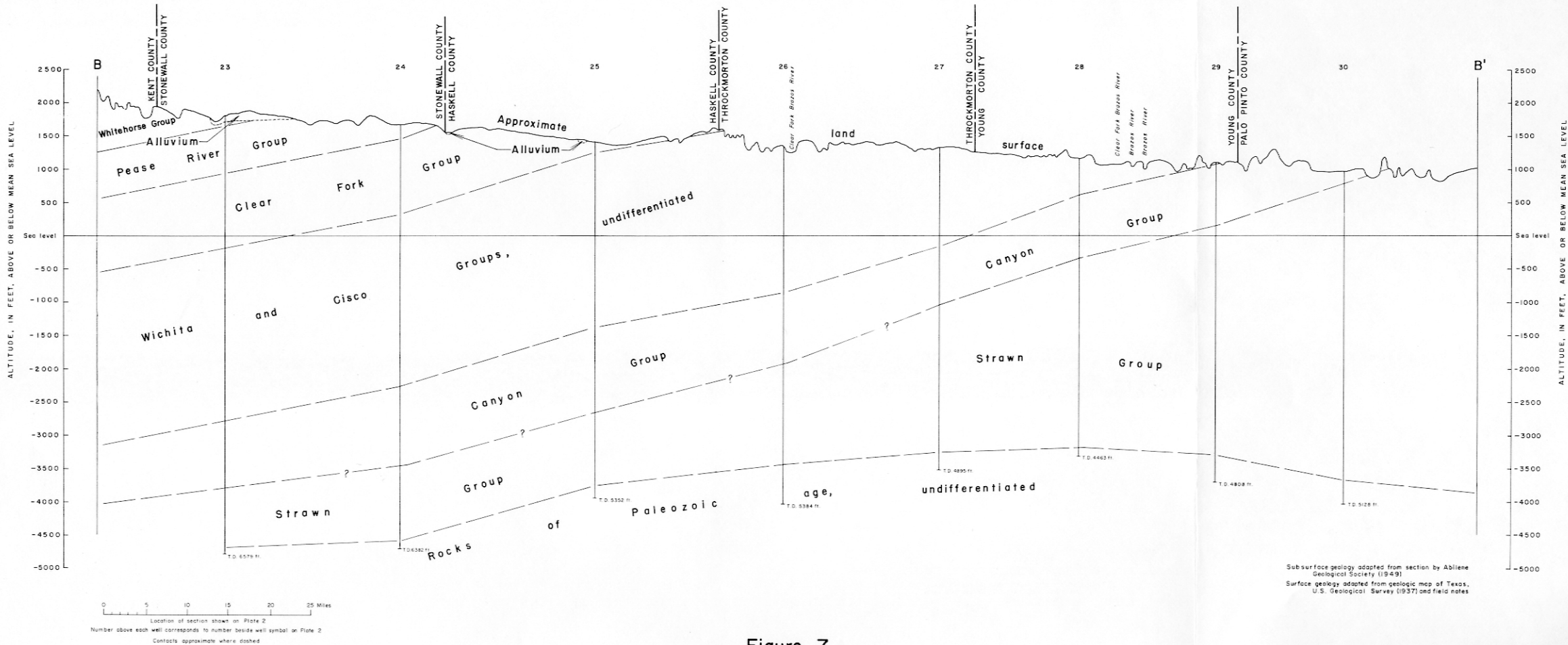
Figure 7 Section B-B', Region II, Brazos River Basin
