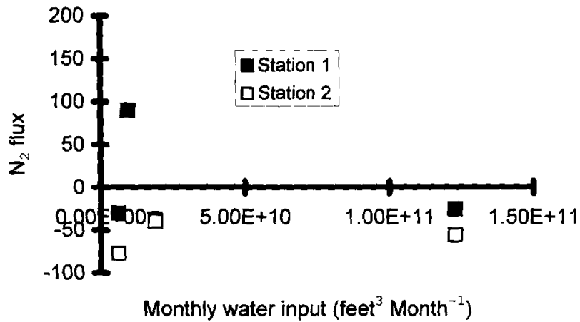
Figure 5. Relationship between freshwater input to Sabine Lake and SOD (a) and N 2 flux (b).
