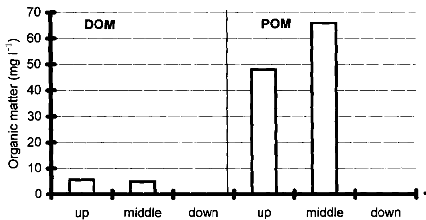
Figure 6. Dissolved organic matter (DOM) and particulated organic matter (POM) concentration in upper, middle, and lower Sabine Lake. The freshwater discharge was 1600 \text{ ft}^3 \text{ sec}^{-1} in low flow season and 16000 \text{ ft}^3 \text{ sec}^{-1} in high flow season. Data from Baskaran et al. 1997.
