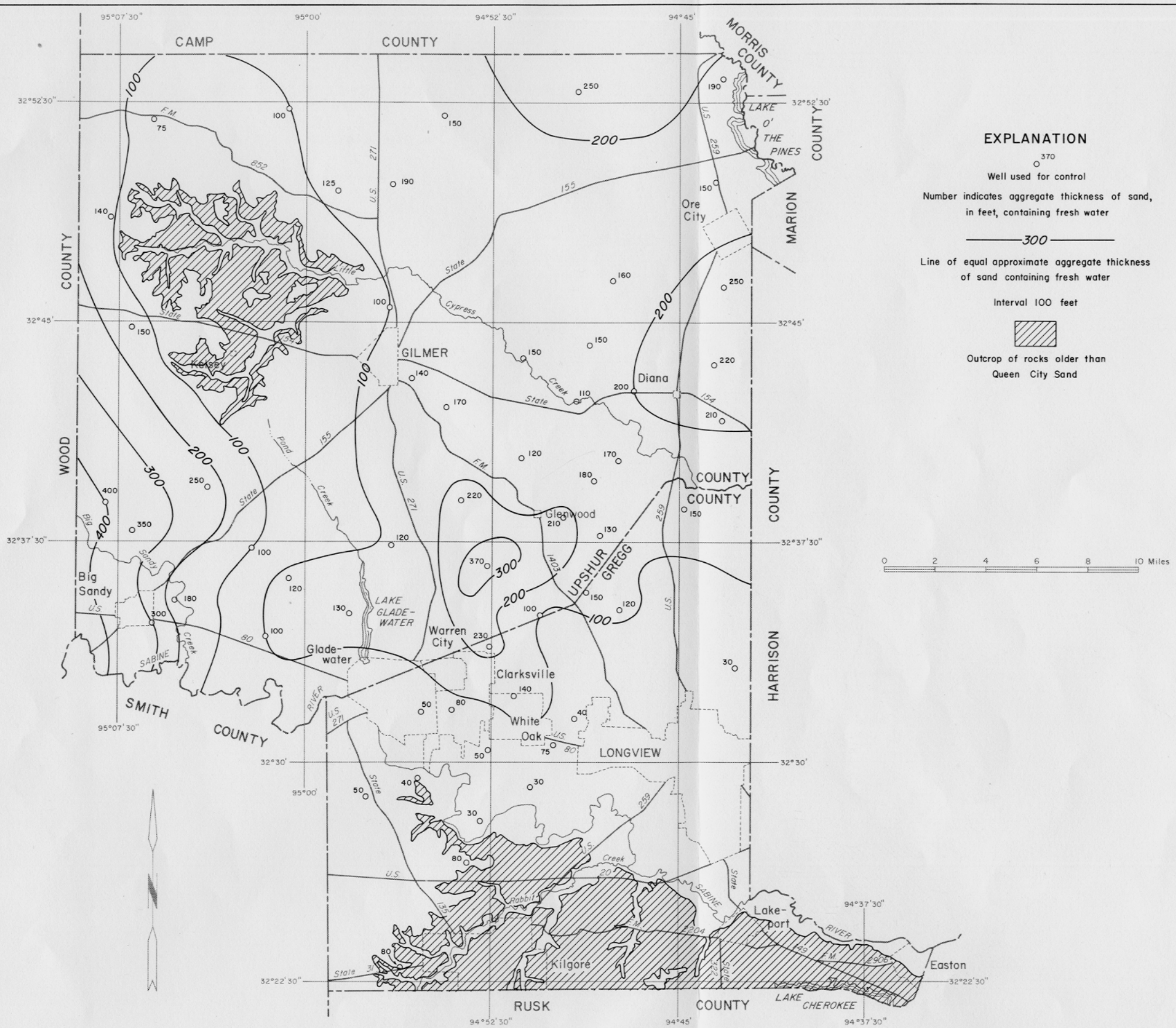
Figure 12 Approximate Thickness of Sand Containing Fresh Water in the Queen City Sand
