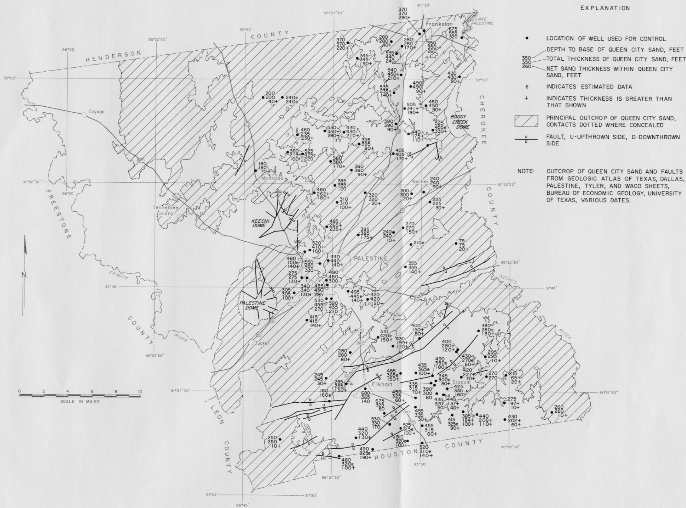
Figure 55 Depth of Base and Thickness of Queen City Sand in Anderson County
