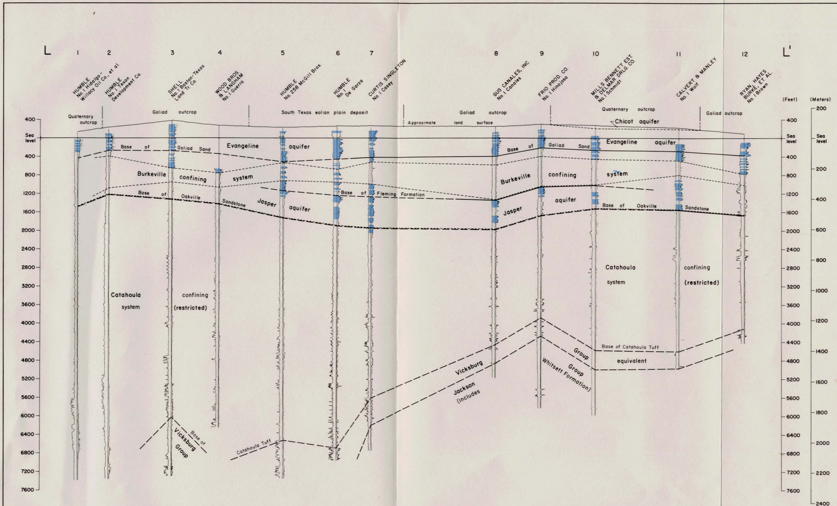
Figure 13 Stratigraphic and Hydrogeologic Section L-L'
