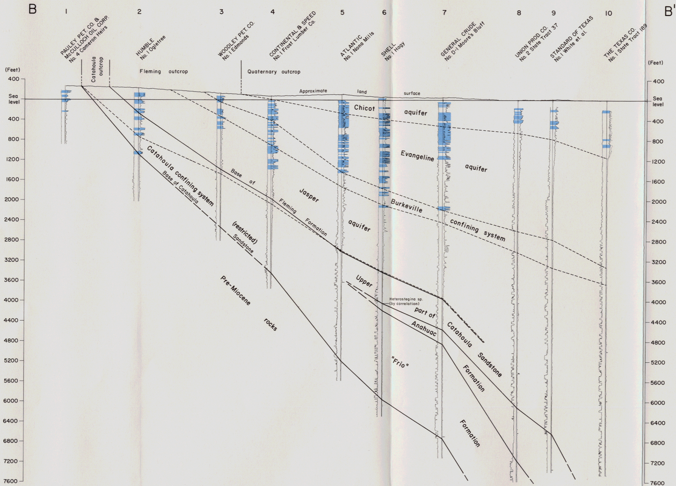
Figure 4 Stratigraphic and Hydrologic Section, B-B'
