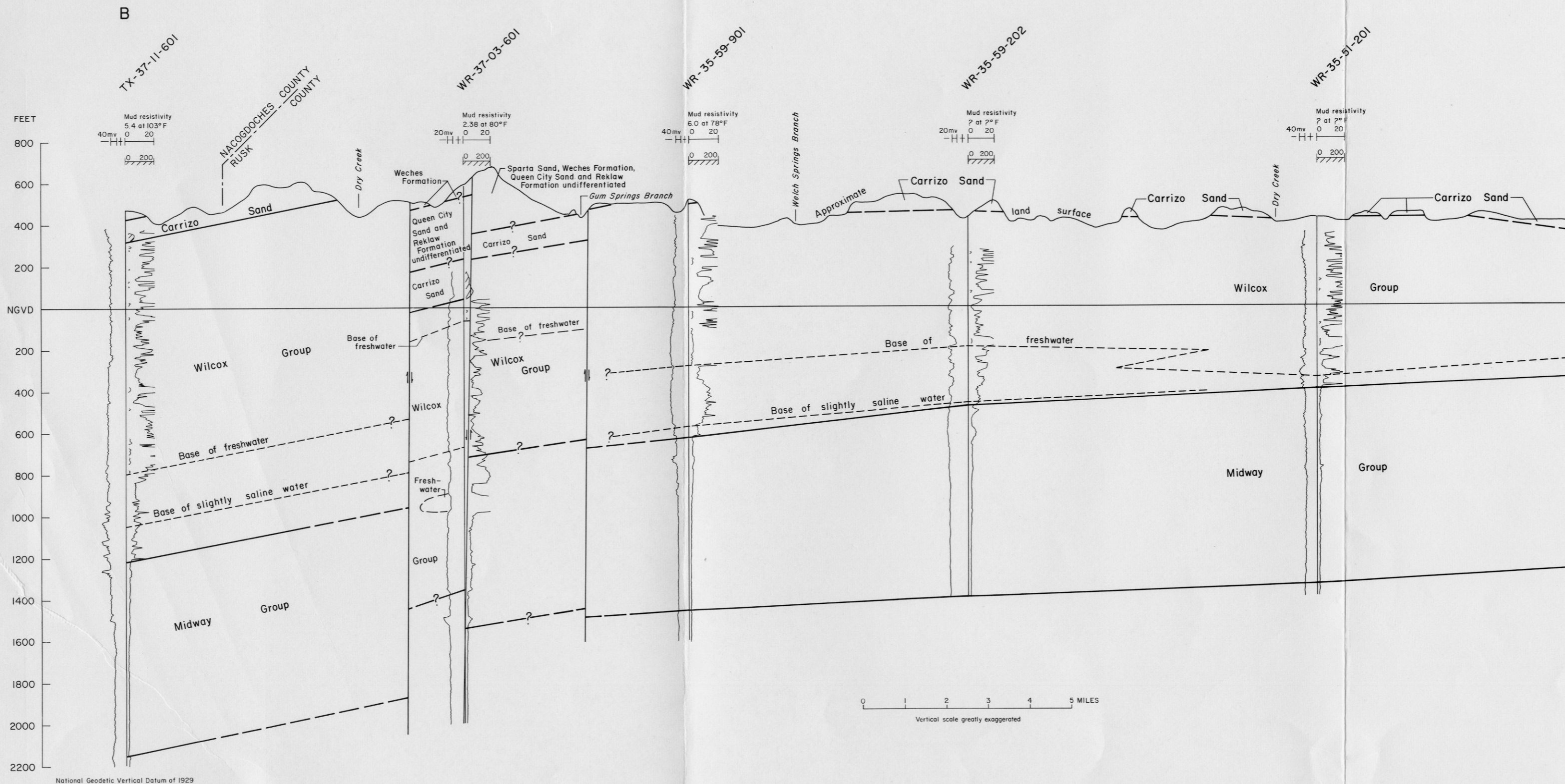
Figure 26 Geologic Section B-B'
