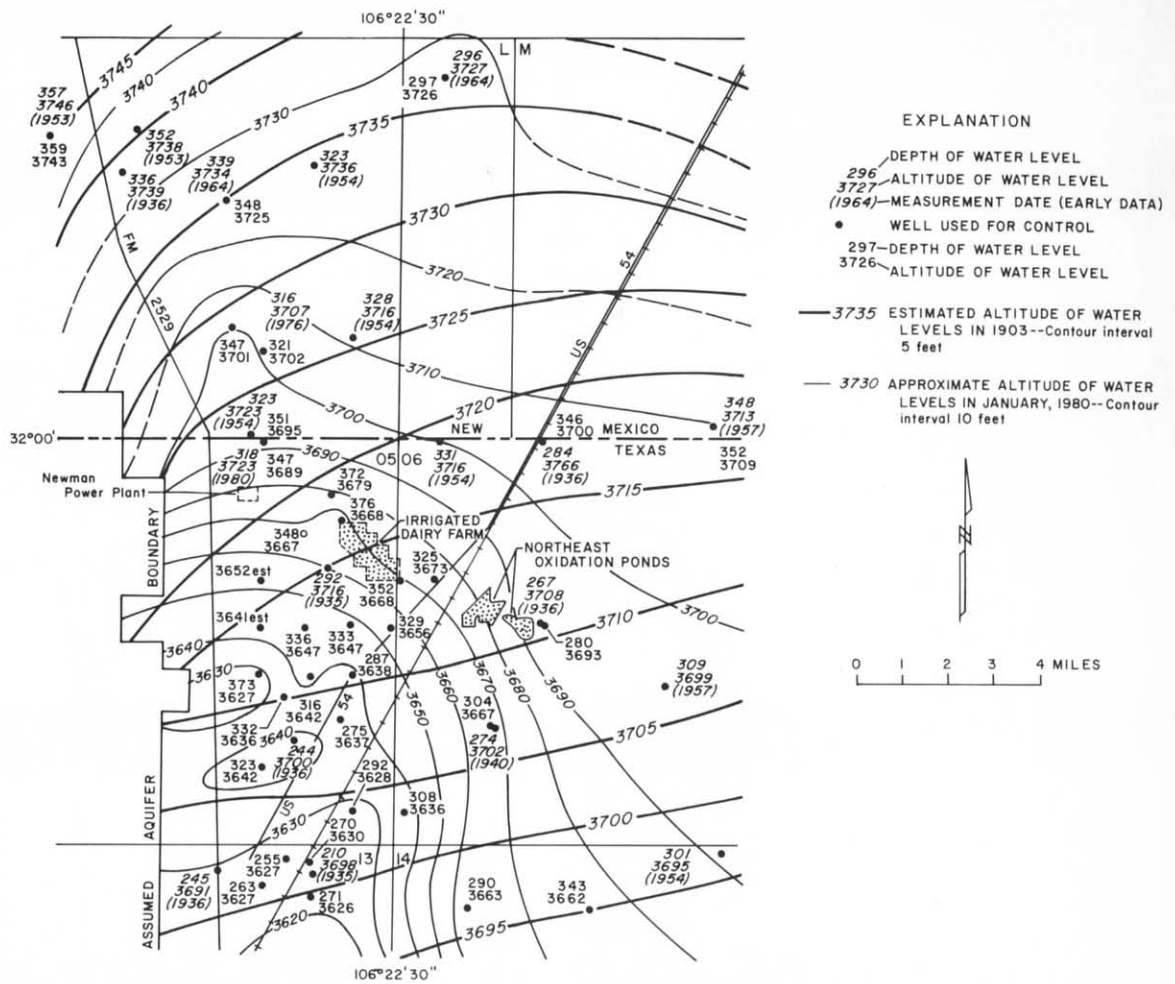
Figure 30.—Depths to Water and Approximate Water-Table Elevations for Early Data and January 1980, in Northeast El Paso and Adjacent Areas in New Mexico
