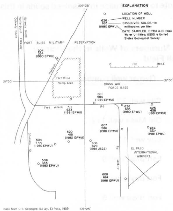
Base from U.S. Geological Survey, El Paso, 1955 Figure 22.—Dissolved-Solids Concentrations in Samples Pumped From Wells in the Vicinity of the Old Mesa Well Field, 1979-81
