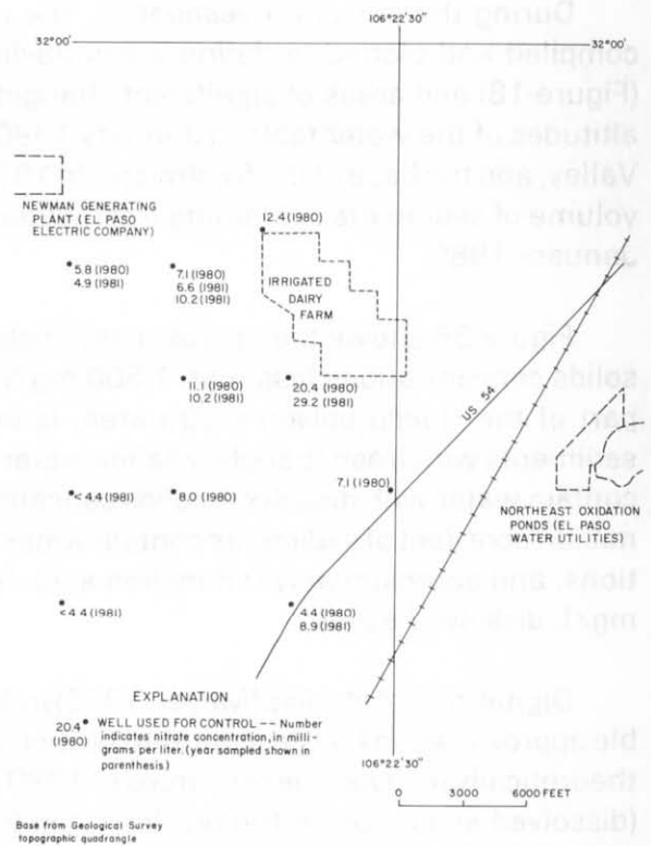
Figure 33.—Concentrations of Nitrate in Water From Wells in the Vicinity of the Dairy Farm, 1980 and 1981
