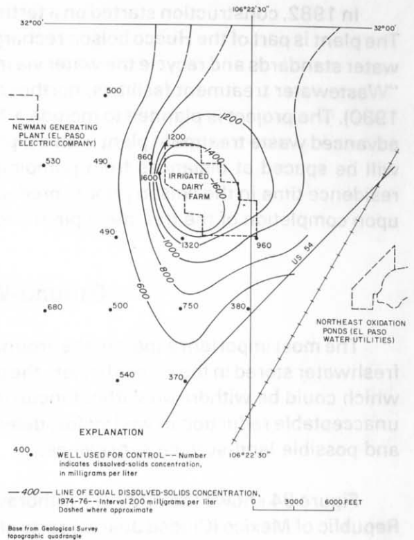
Figure 32b.—Approximate Areal Distribution of the Dissolved-Solids Concentration in Water From Wells in the Vicinity of the Dairy Farm, 1974-76
