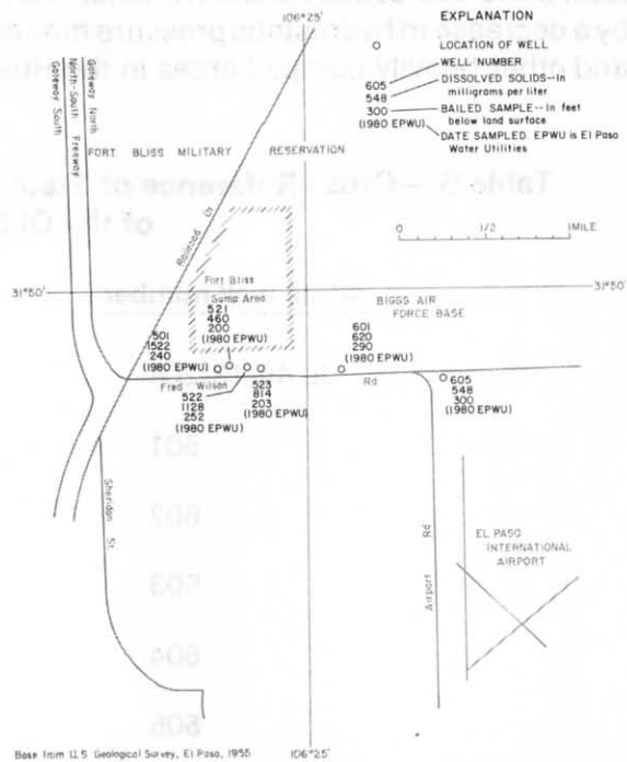
Base from U.S. Geological Survey, El Paso, 1955 Figure 23.—Dissolved-Solids Concentrations in Samples Bailed From Wells in the Vicinity of the Old Mesa Well Field, 1980
