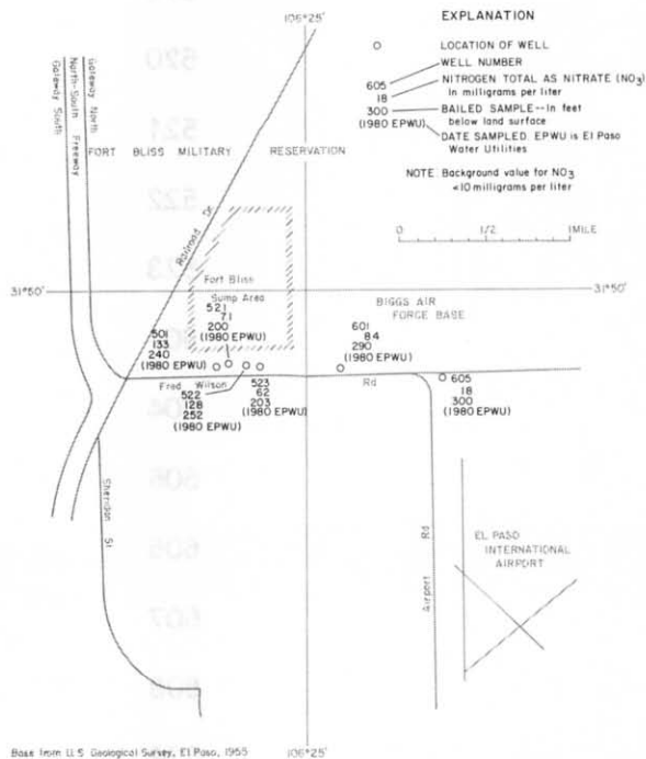
Base from U.S. Geological Survey, El Paso, 1955 Figure 25.—Total Nitrogen Concentrations in Samples Bailed From Wells in the Vicinity of the Old Mesa Well Field, 1980
