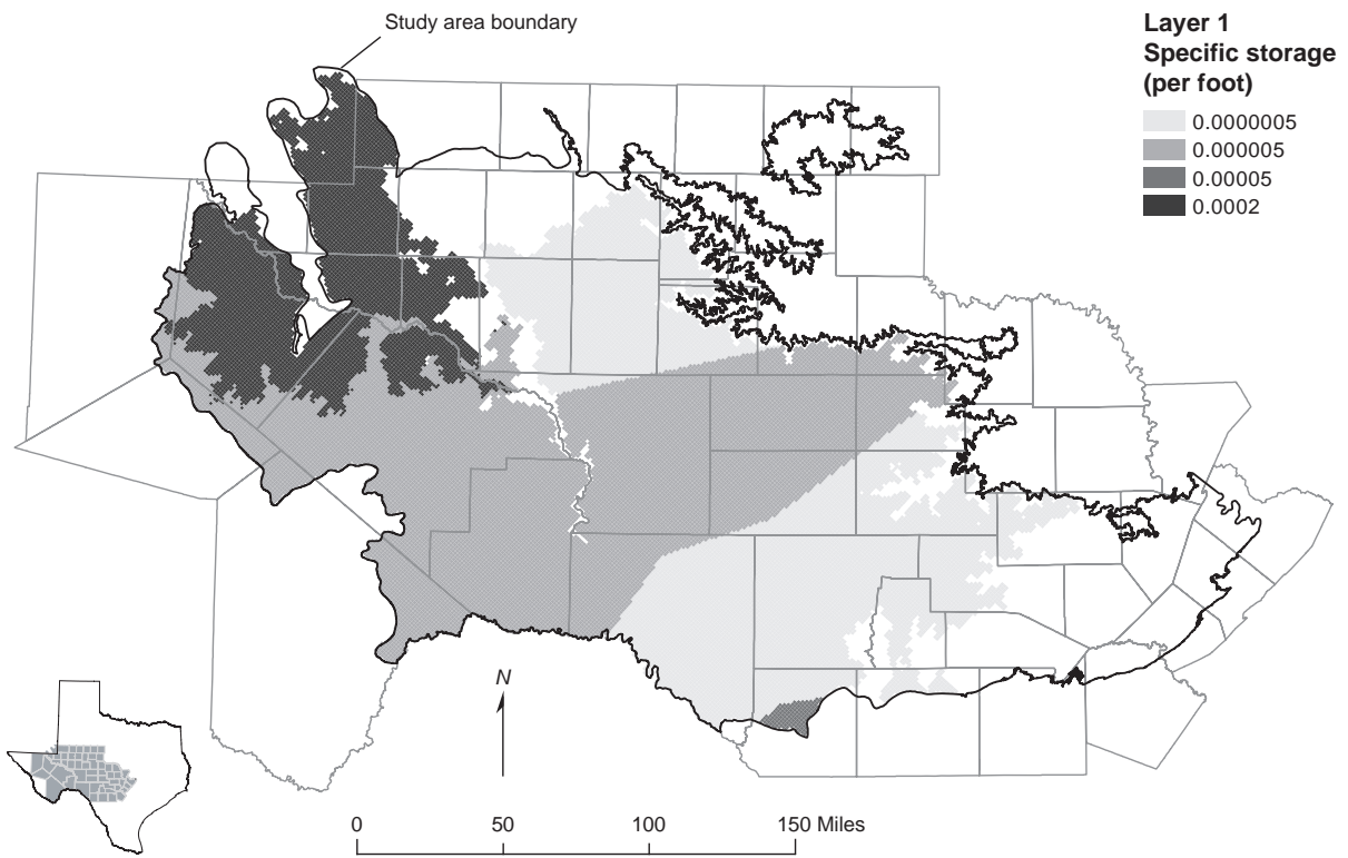
Figure 10-5. Specific storage for layer 1 used within model.
