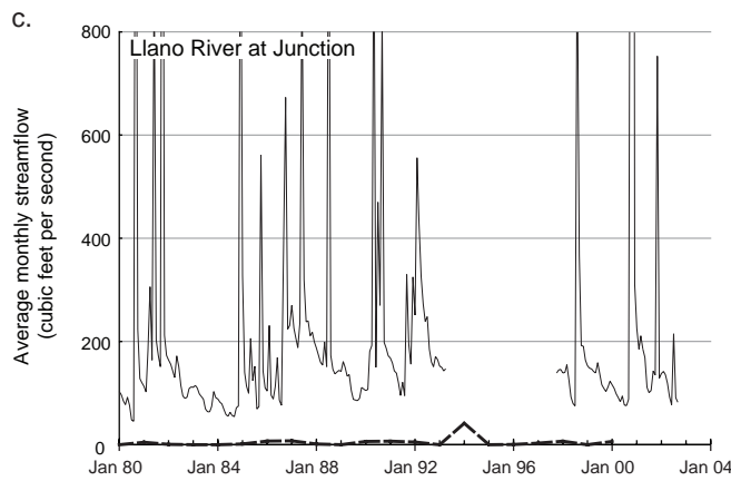
Figure 10-8. Comparison of simulated groundwater discharge to perennial streams for the 1980–2000 transient model (dashed line) and measured streamflow.
