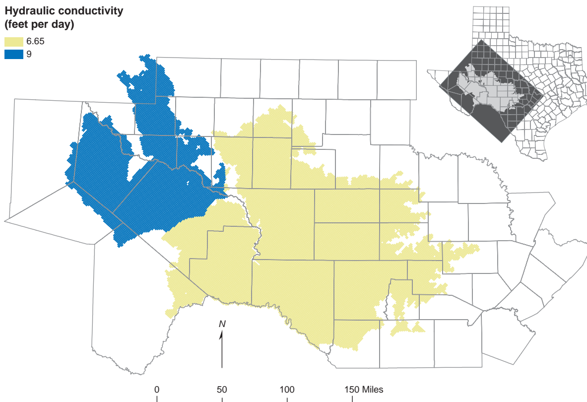
Figure 7-4. Zoned hydraulic conductivity for layer 1 used within model.
