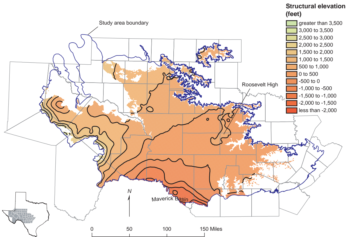
Figure 5-10. Structural base of the Edwards Group.
