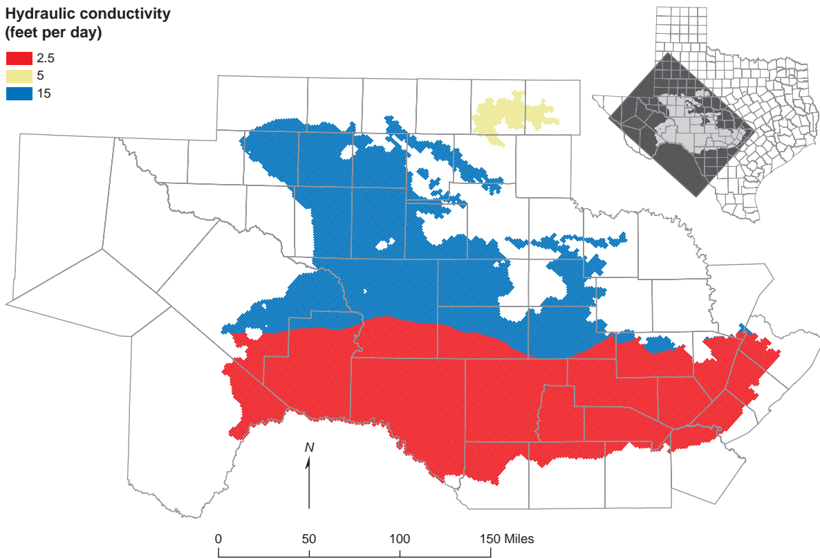
Figure 7-5. Zoned hydraulic conductivity for layer 2 used within model.
