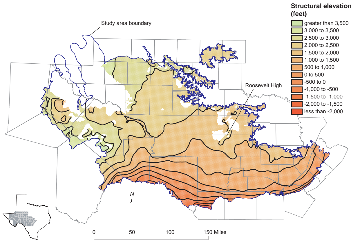
Figure 5-9. Structural base of the Trinity Group.
