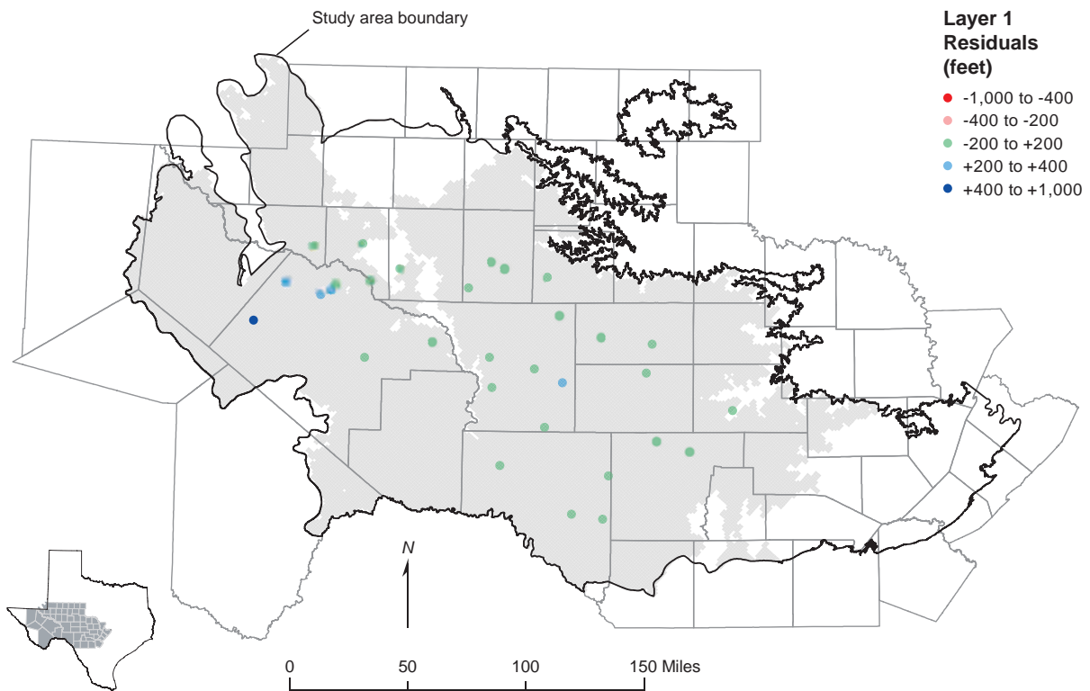
Figure 10-9. Spatial comparison of simulated and measured water levels in layer 1 of the transient model for the 2000 annual stress period. Residuals are the difference between simulated and measured water levels.
