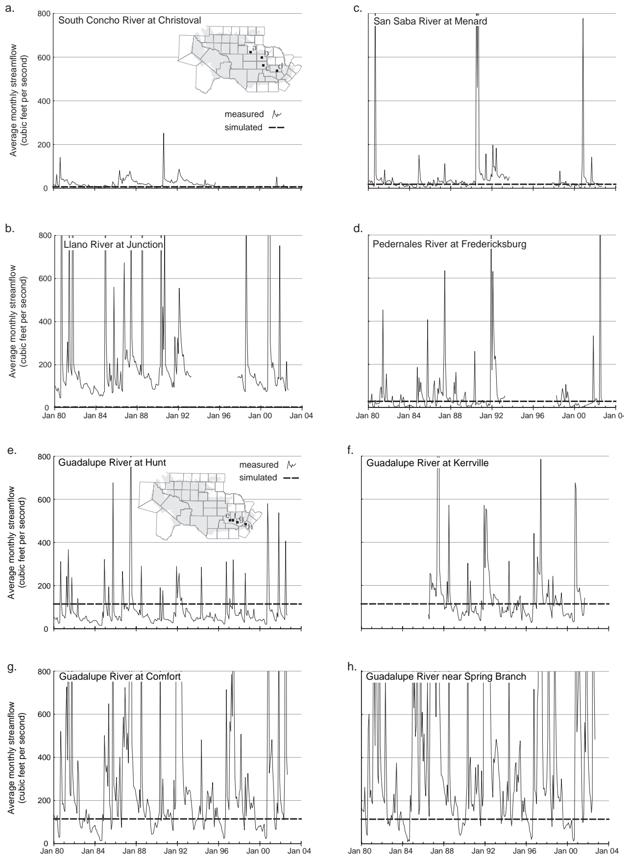
Figure 9-8. Comparison of simulated groundwater discharge to perennial streams for the 1980 steady-state model (dashed line) and measured streamflow.
