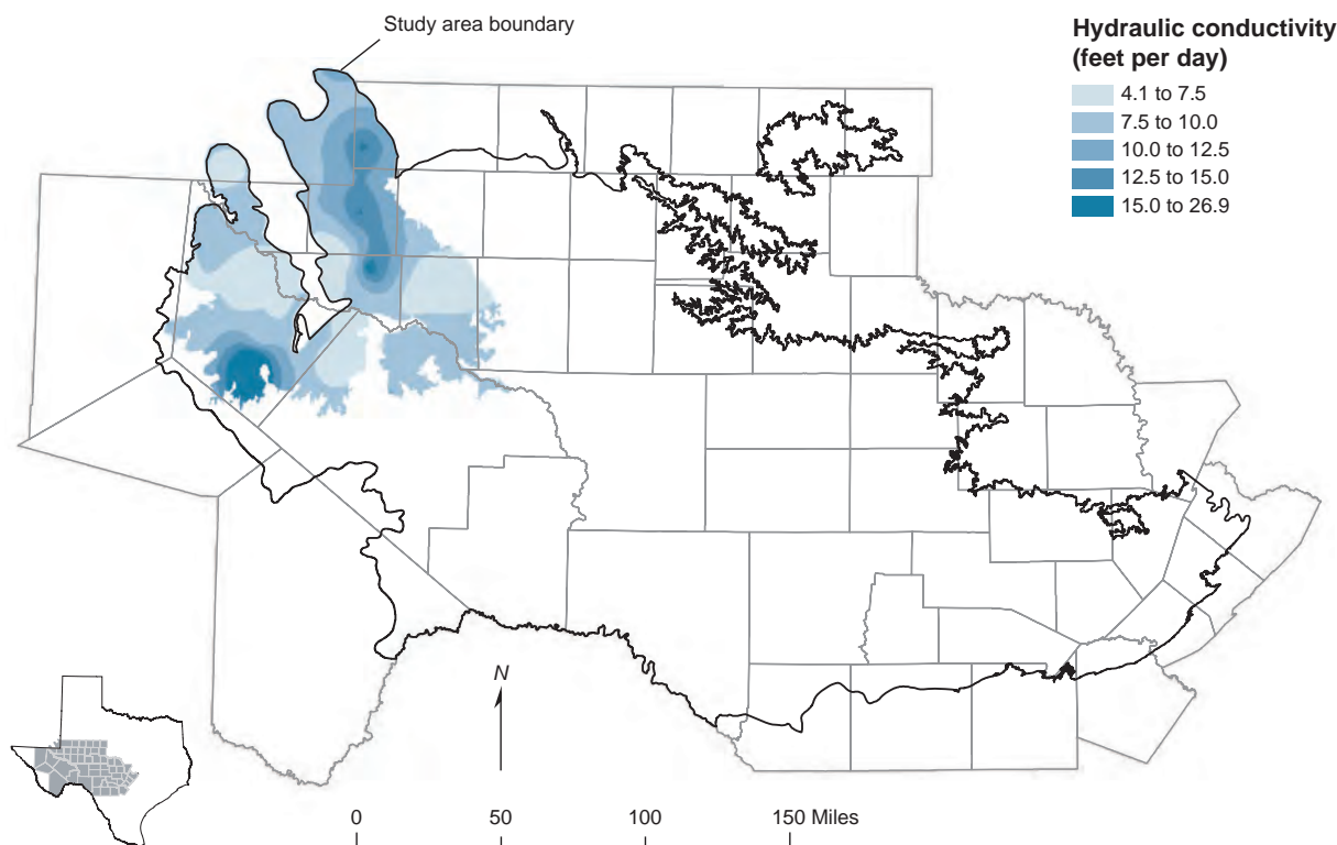
Figure 5-20. Interpolated hydraulic conductivity for the Pecos Valley Aquifer.
