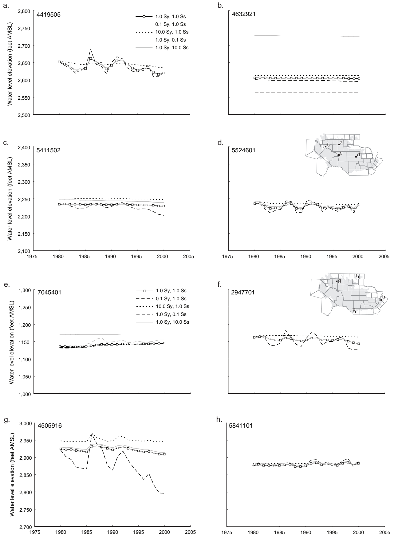
Figure 10-12. Sensitivity of model to specific yield and specific storage.
