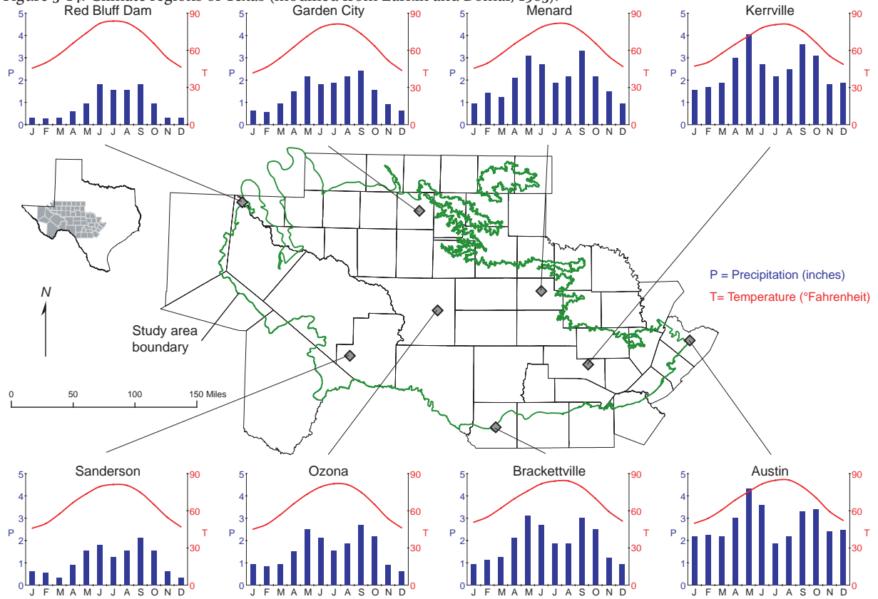
Figure 3-14. Climate regions of Texas (modified from Larkin and Bomar, 1983).
