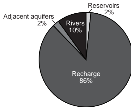
Figure 9-9. Groundwater inflows and outflows of the water budget for the 1980 steady-state model.
