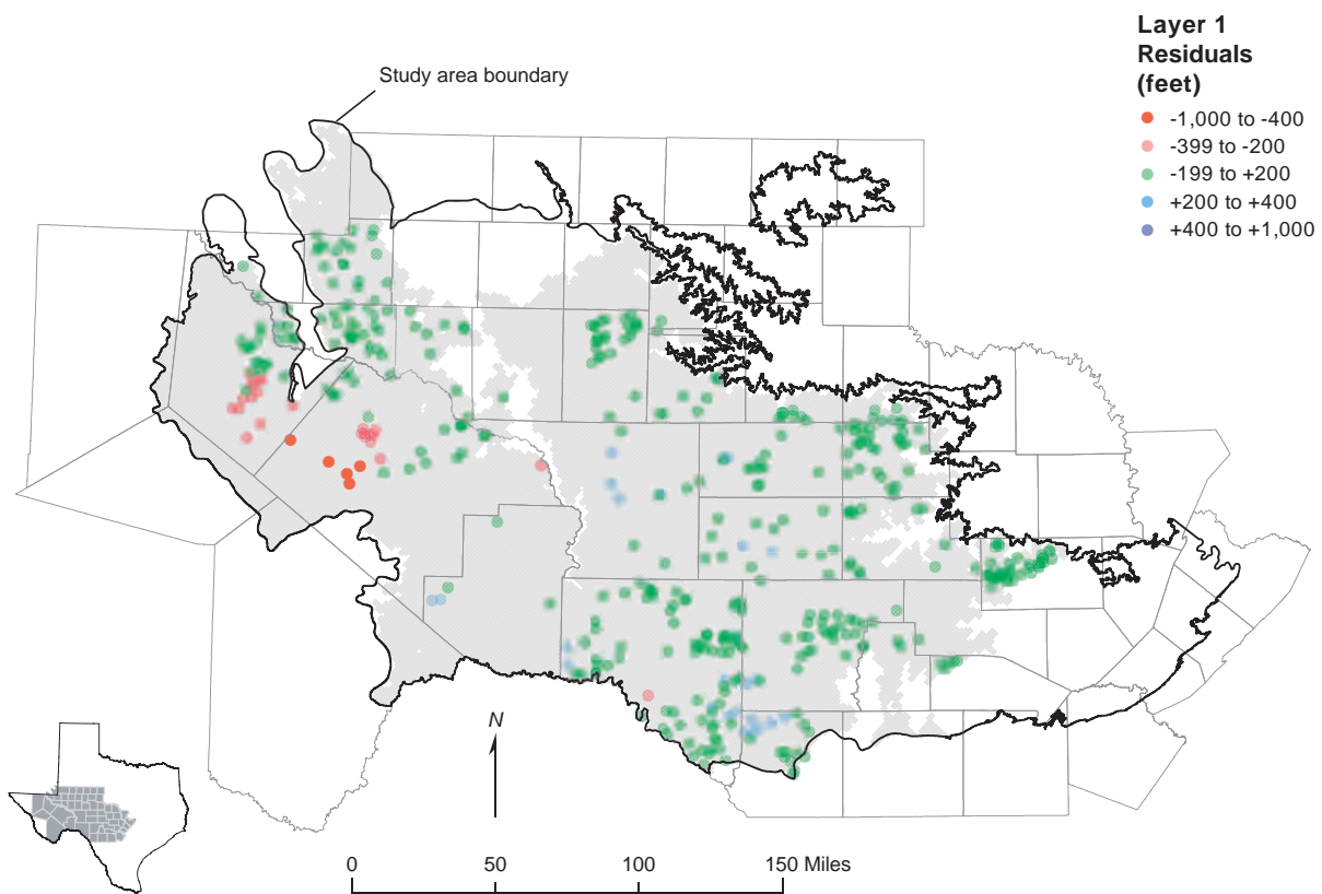
Figure 9-5. Spatial comparison of simulated and measured water levels in layer 1 for the 1980 steady-state model. Residuals are the difference between simulated and measured water levels.
