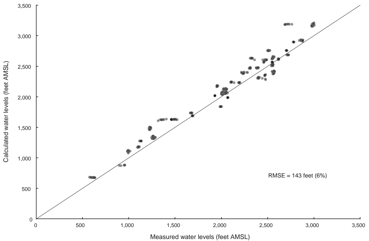
Figure 10-11. Cross plot comparison of simulated and measured water levels for both layers 1 and 2 of the (1980–2000) transient model.
