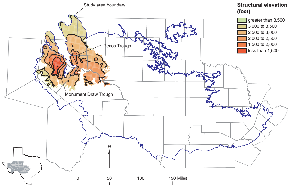
Figure 5-11. Structural base of the Pecos Valley.
