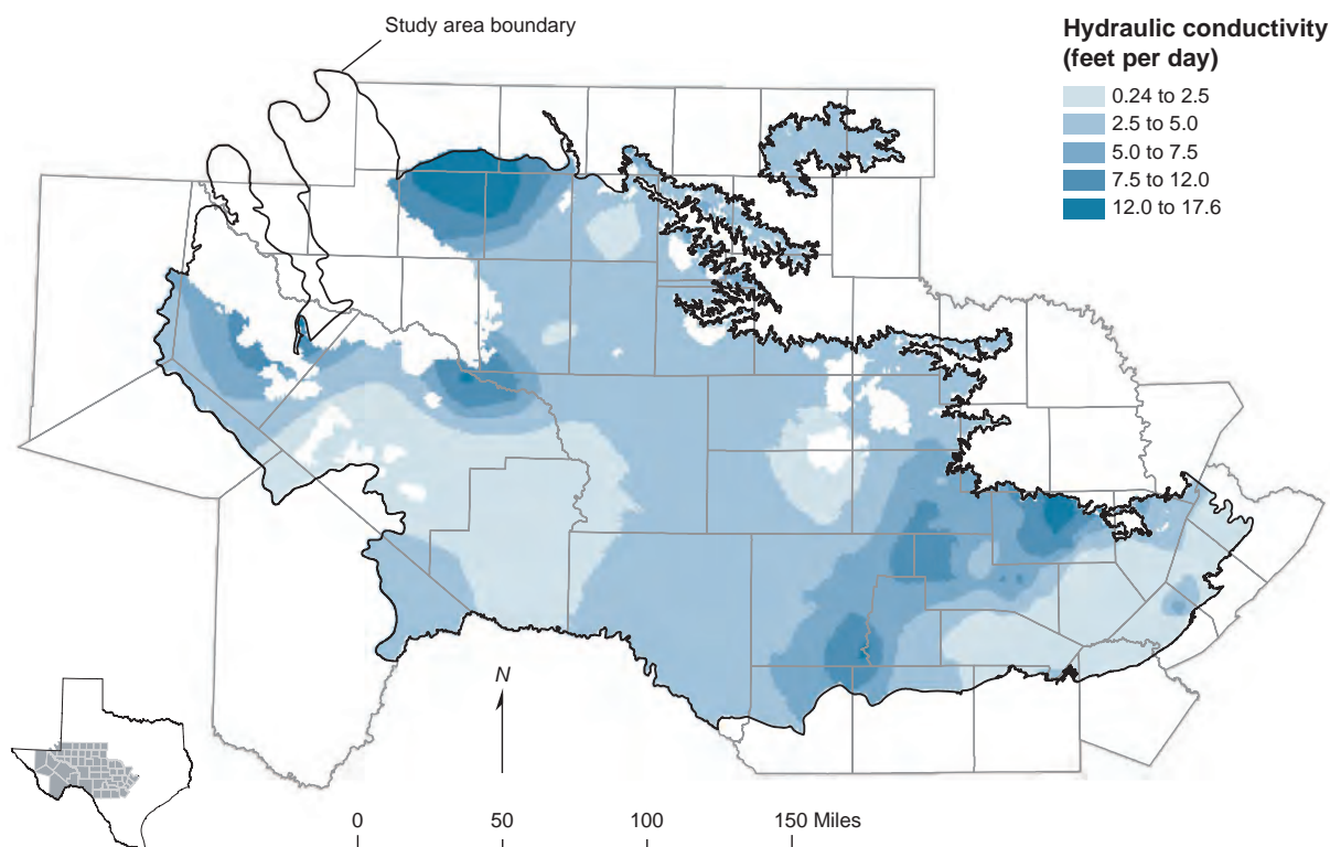
Figure 5-18. Interpolated hydraulic conductivity for the Trinity hydrostratigraphic unit of the Edwards-Trinity (Plateau) Aquifer.
