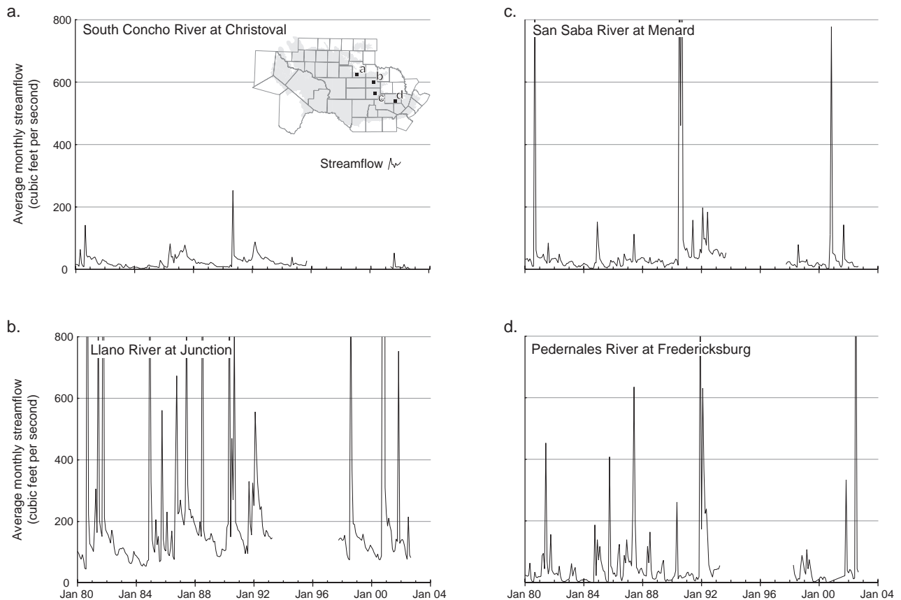
Figure 5-23. Streamflow hydrographs for major perennial streams over the Edwards-Trinity (Plateau) and Pecos Valley aquifers and Hill Country part of the Trinity Aquifer.
