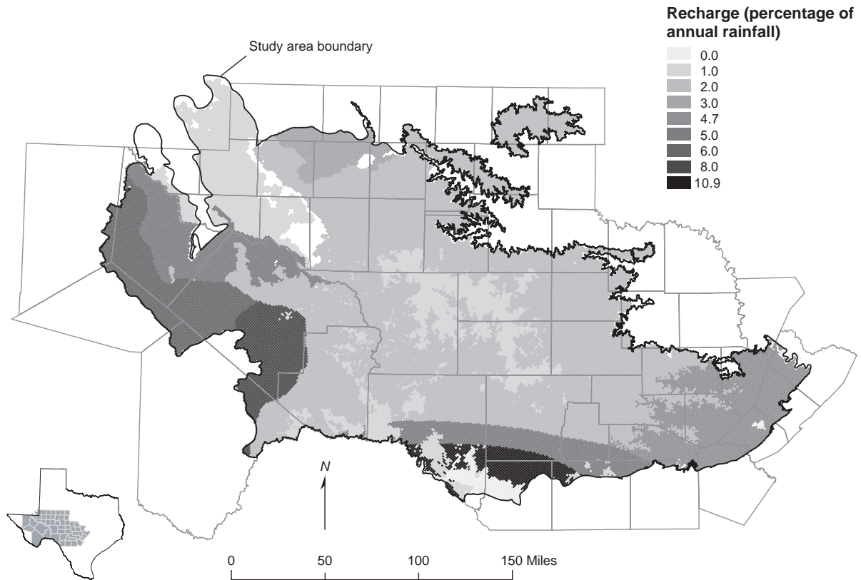
Figure 9-4. Model calibrated zones of recharge expressed as a percentage of annual rainfall.
