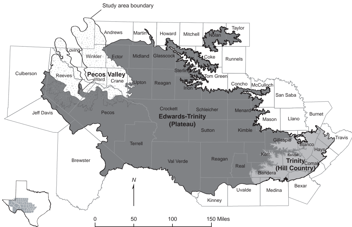
Figure 3-3. Spatial extents of the Edwards-Trinity (Plateau) and Pecos Valley aquifers and Hill Country part of the Trinity Aquifer.
