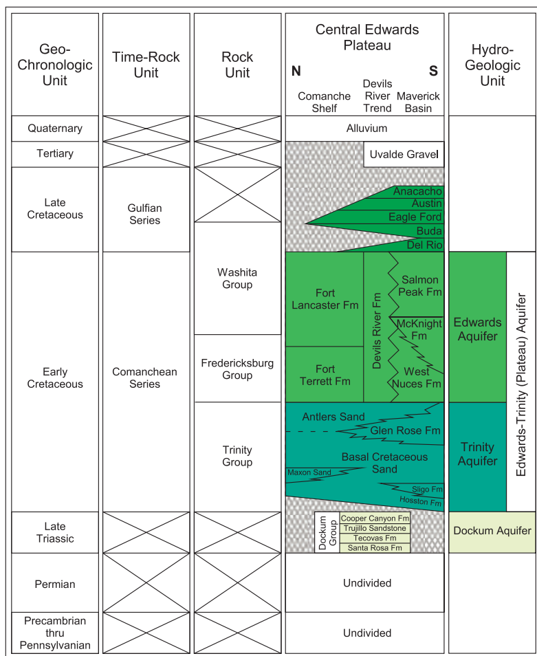
Figure 5-5. Hydrostratigraphic chart of the central Edwards Plateau region. Fm=formation
