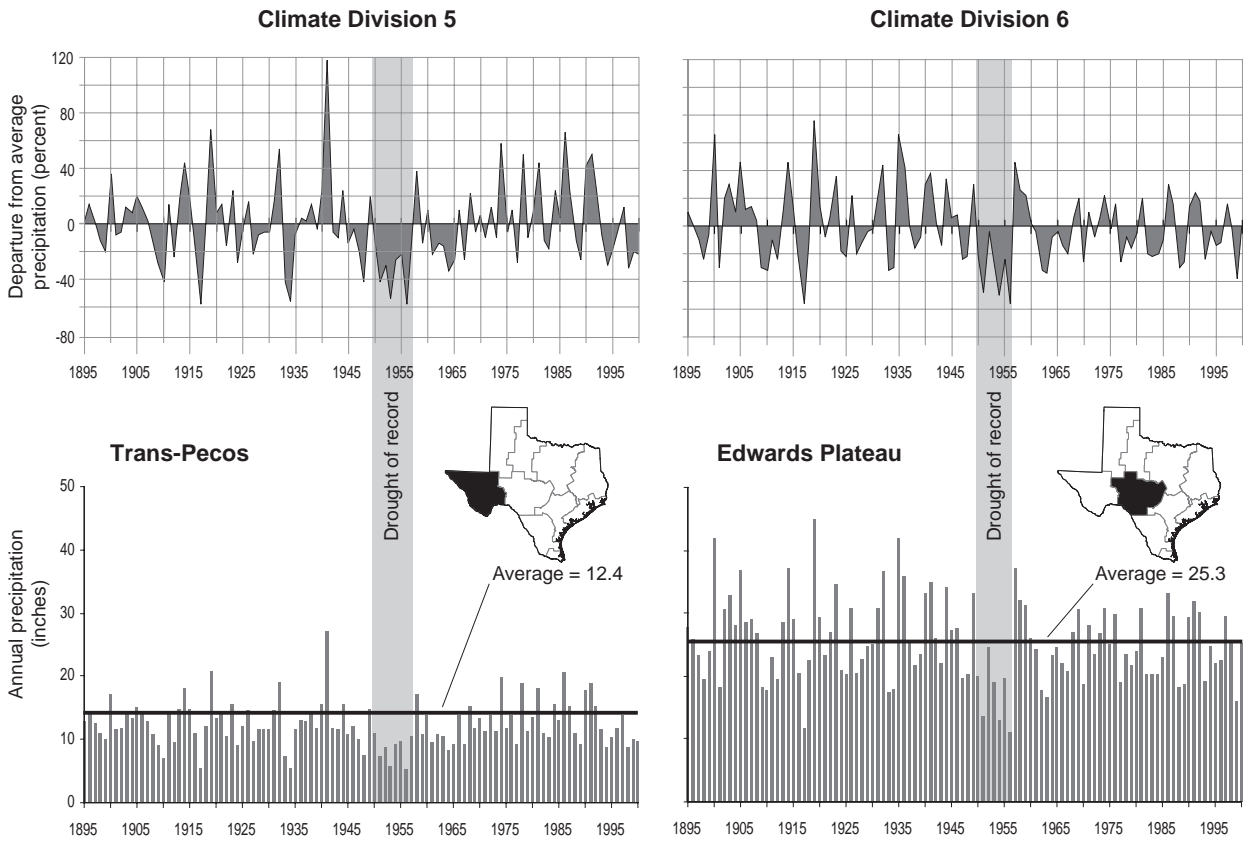
Figure 3-20. Annual precipitation and departure from average annual precipitation for 1895–2003 in the Trans-Pecos and Edwards Plateau climate divisions.
