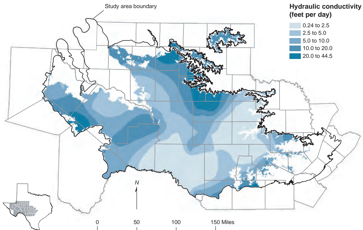
Figure 5-19. Interpolated hydraulic conductivity for the Edwards hydrostratigraphic unit of the Edwards-Trinity (Plateau) Aquifer.
