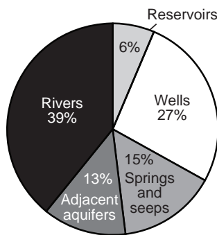
Figure 9-9. Groundwater inflows and outflows of the water budget for the 1980 steady-state model.
