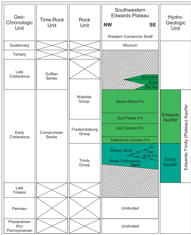
Figure 5-7. Hydrostratigraphic chart of the southwestern Edwards Plateau, Stockton Plateau region. Fm=formation
