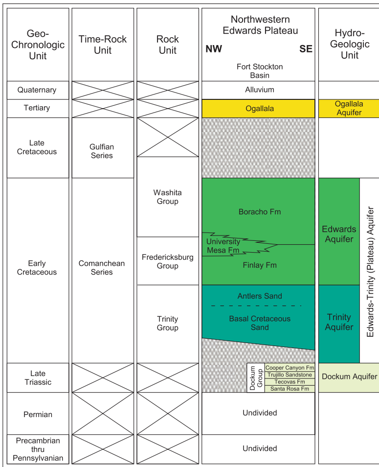
Figure 5-6. Hydrostratigraphic chart of the northwestern Edwards Plateau, Llano Estacado region. Fm=formation
