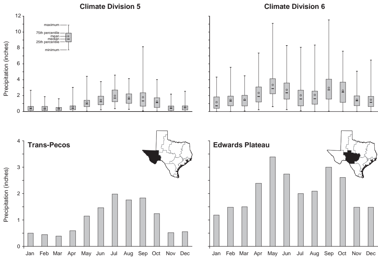
Figure 3-17. Monthly precipitation statistics for 1895–2003 in the Trans-Pecos and Edwards Plateau climate divisions.
