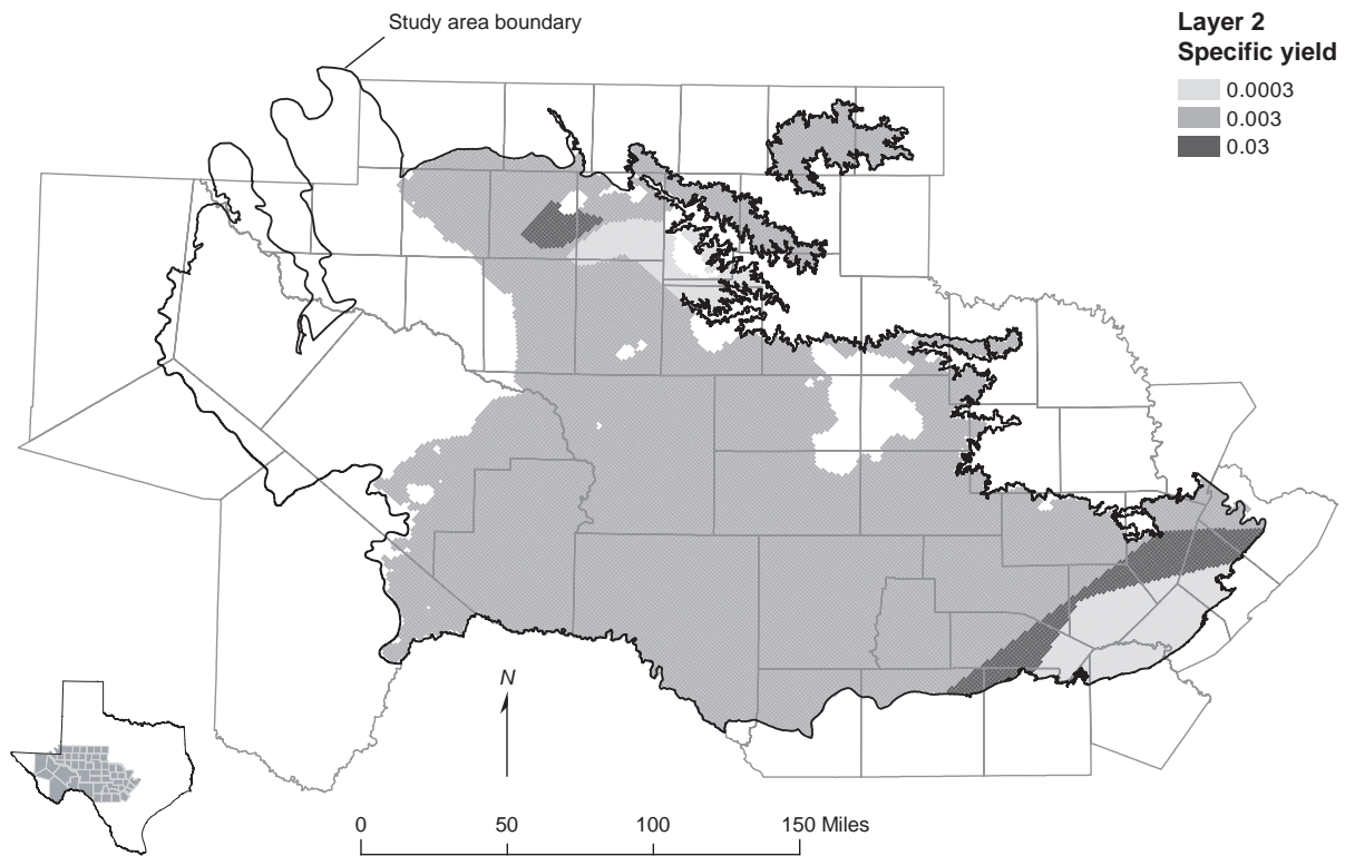
Figure 10-4. Specific yield for layer 2 used within model.
