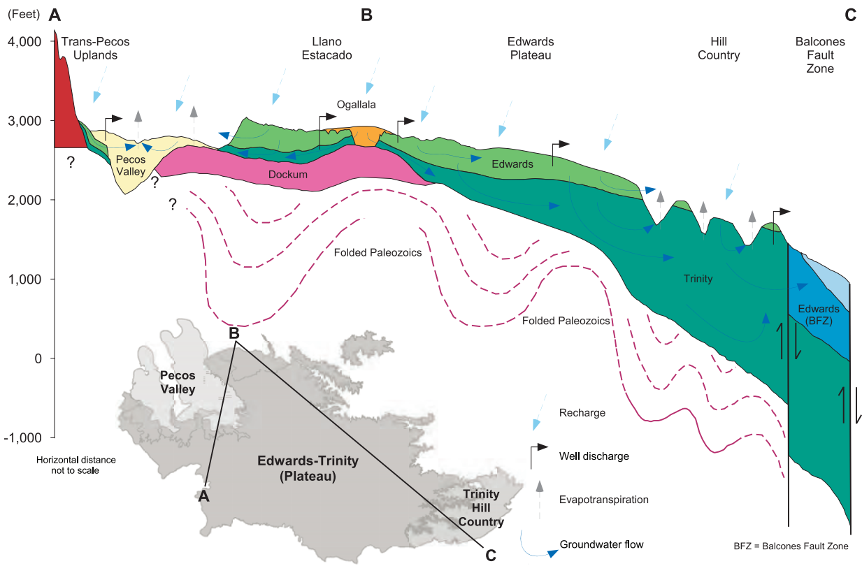
Figure 6-1. Conceptual model of the Edwards-Trinity (Plateau) and Pecos Valley aquifers and Hill Country part of the Trinity Aquifer.
