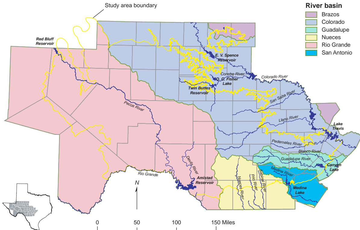
Figure 3-9. Major streams and drainage basins of the study area.
