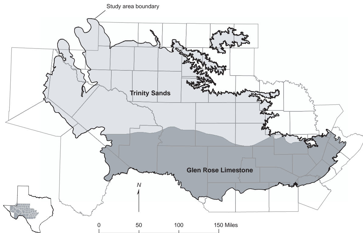
Figure 5-21. Delineation between the Trinity Sands and Glen Rose Limestone extents of the Trinity hydrostratigraphic unit of the Edwards-Trinity (Plateau) Aquifer.
