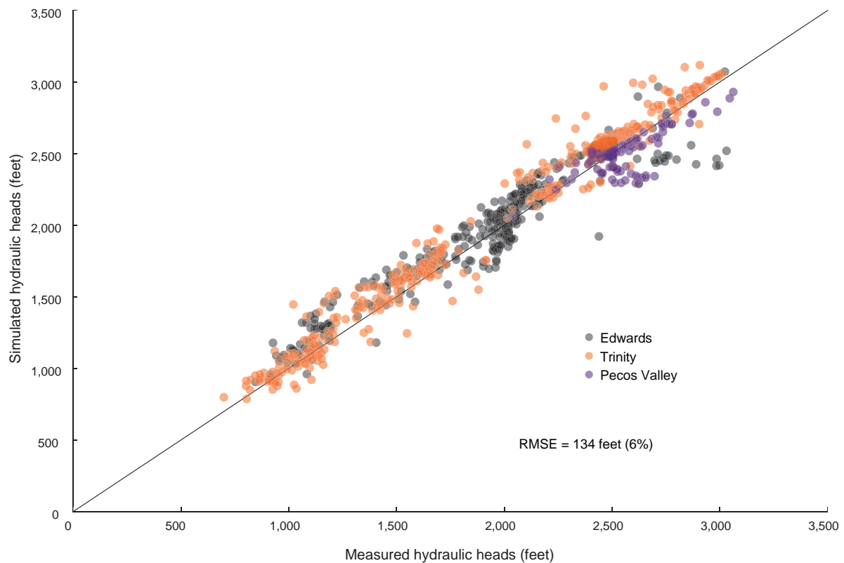
Figure 9-7. Cross plot comparison of simulated and measured water levels for layers 1 and 2 for the 1980 steady-state model. RMSE=root mean square error.
