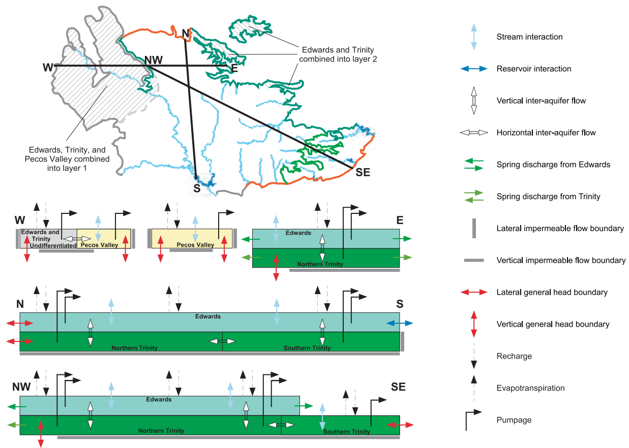
Figure 6-2. Block diagram of the Edwards-Trinity (Plateau), Trinity (Hill Country), and Pecos Valley aquifers.
