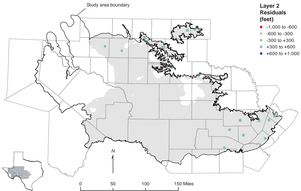
Figure 10-10. Spatial comparison of simulated and measured water levels in layer 2 of the transient model for the 2000 annual stress period. Residuals are the difference between simulated and measured water levels.
