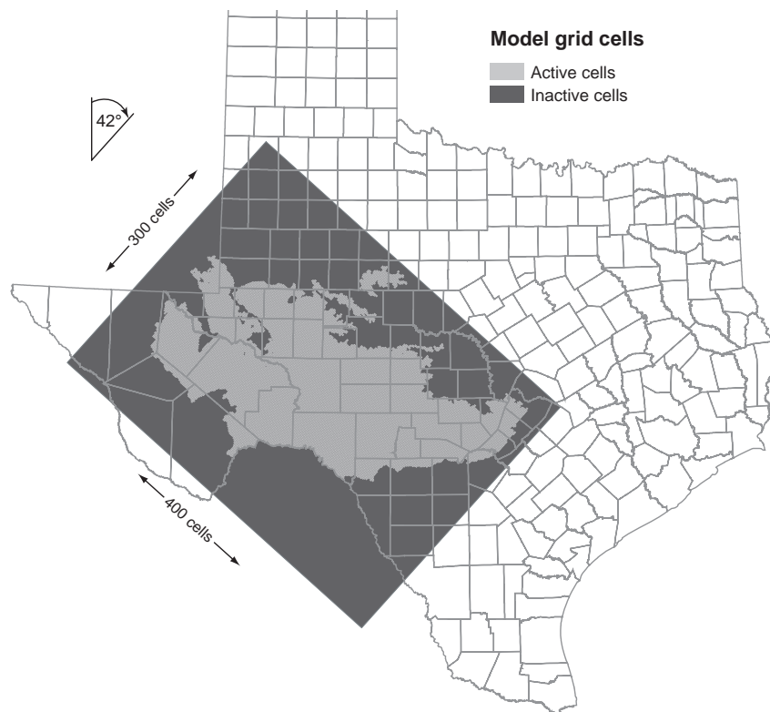
Figure 7-1. Model grid location and orientation showing active and inactive cells.
