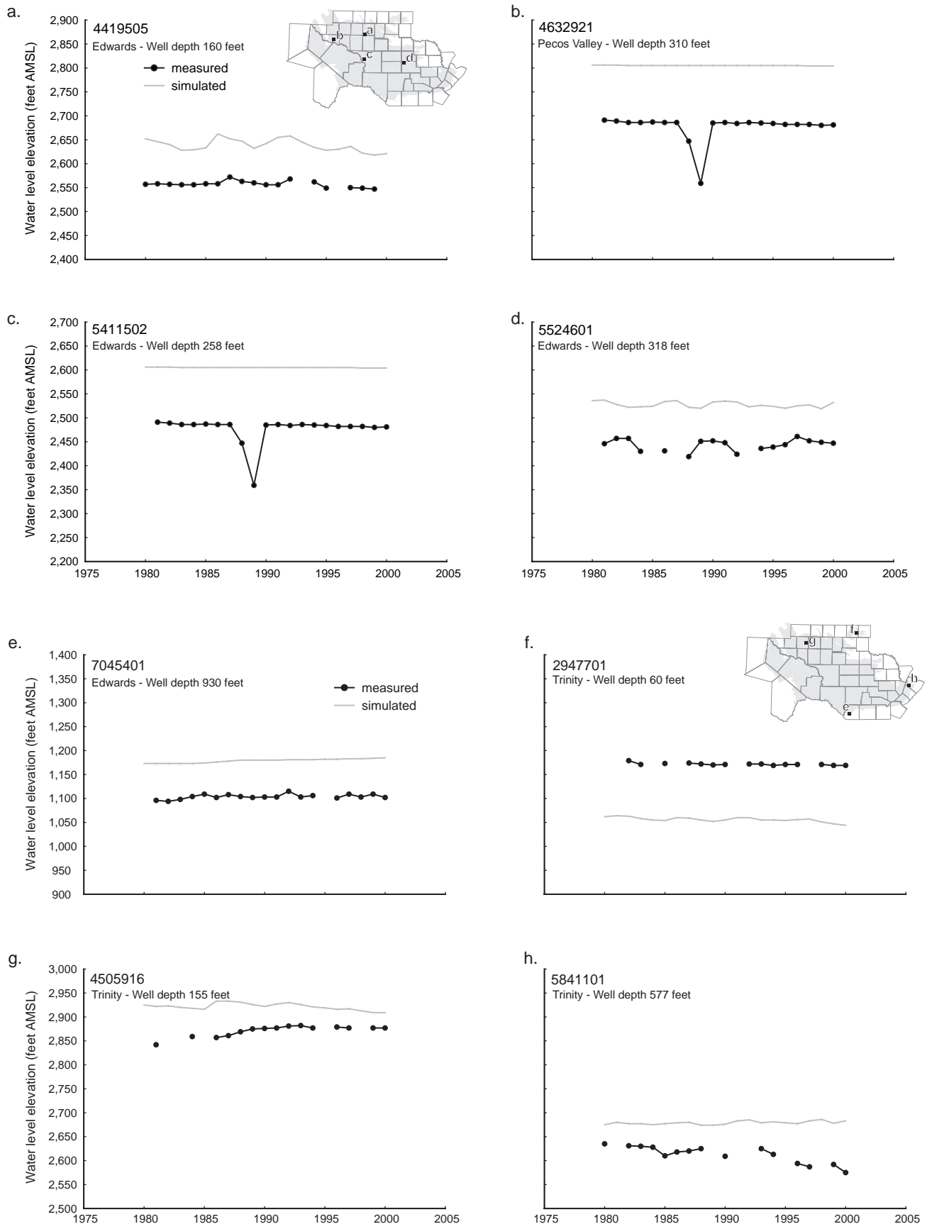
Figure 10-7. Measured and simulated water level fluctuations for the period 1980–2000. AMSL=above mean sea level
