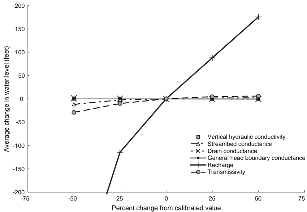
Figure 9-11. Sensitivity of numerically predicted water levels for 1980.
