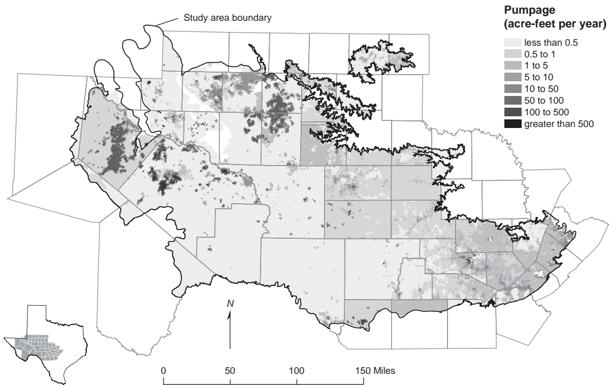
Figure 10-2. Total pumping volumes assigned per grid cell for 2000.
