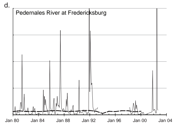
Figure 10-8. Comparison of simulated groundwater discharge to perennial streams for the 1980–2000 transient model (dashed line) and measured streamflow.
