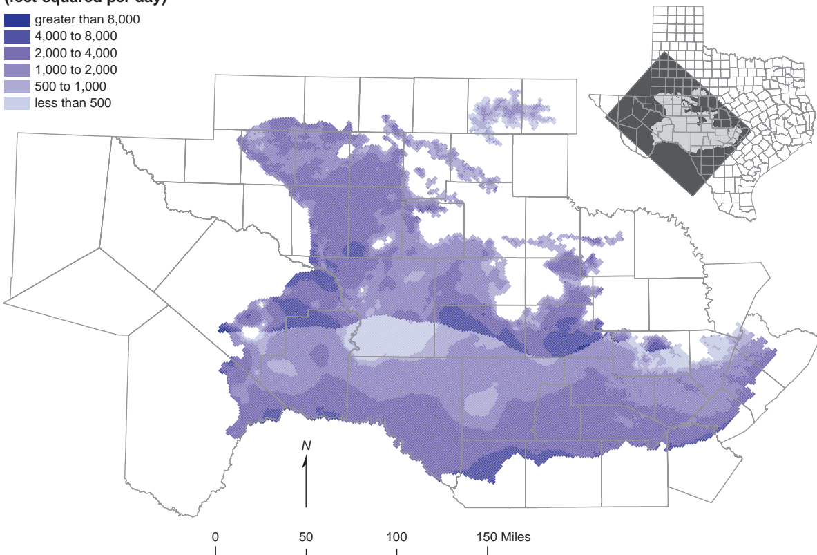
Figure 7-7. Transmissivity for layer 2 used within model.
