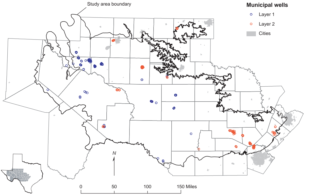
Figure 7-9. Location of municipal well fields used within the model.
