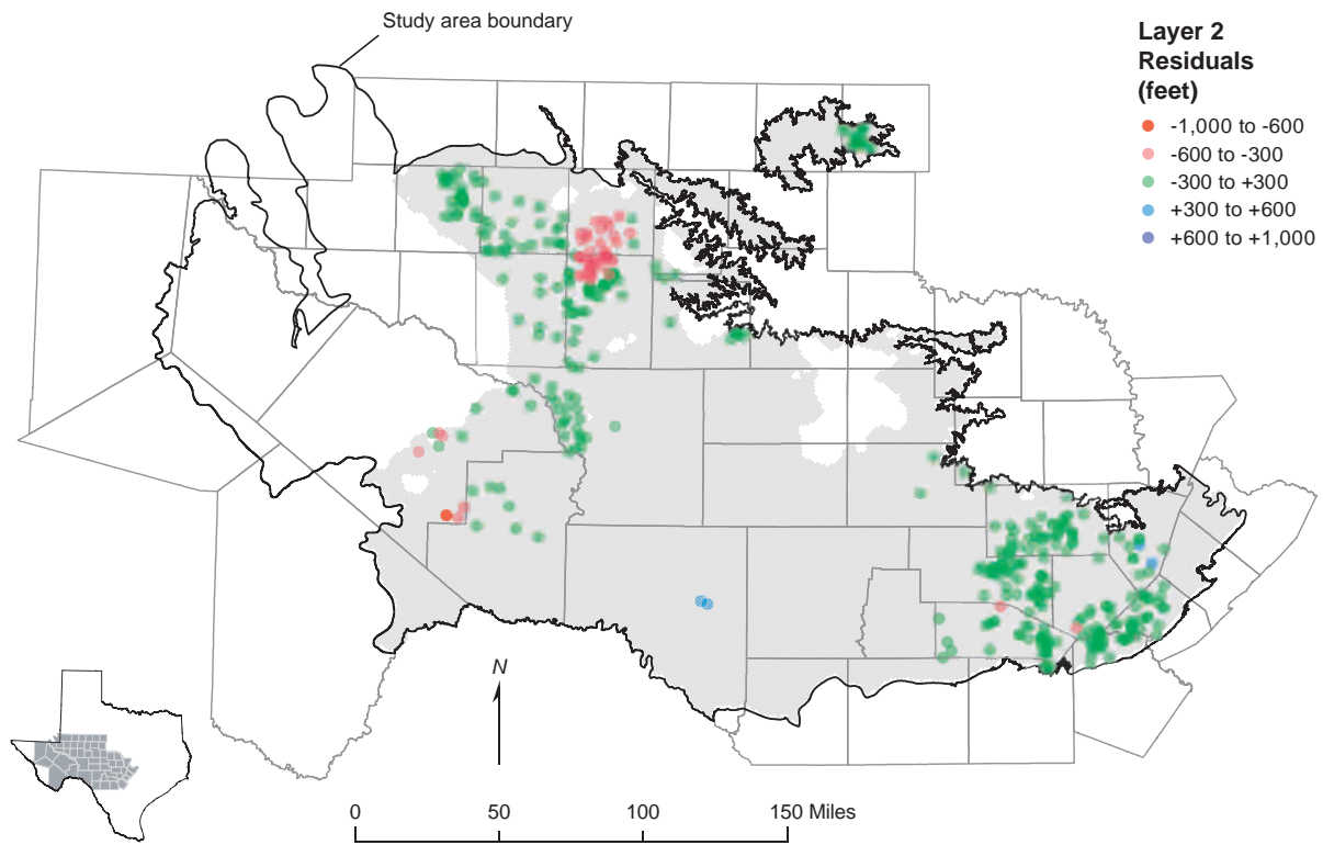
Figure 9-6. Spatial comparison of simulated and measured water levels in layer 2 for the 1980 steady-state model. Residuals are the difference between simulated and measured water levels.
