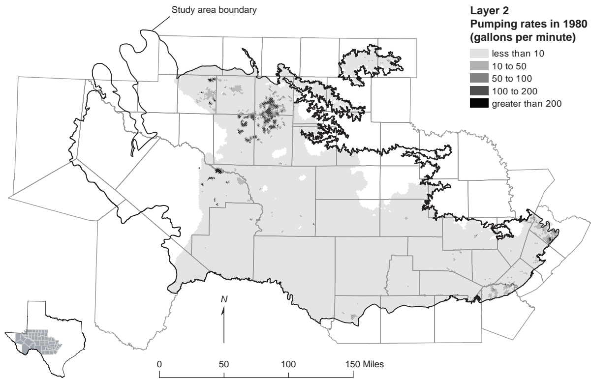
Figure 9-3. Total 1980 pumping volumes for layer 2 distributed within the model grid.
