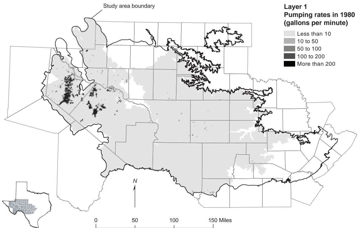
Figure 9-2. Total 1980 pumping volumes for layer 1 distributed within the model grid.
