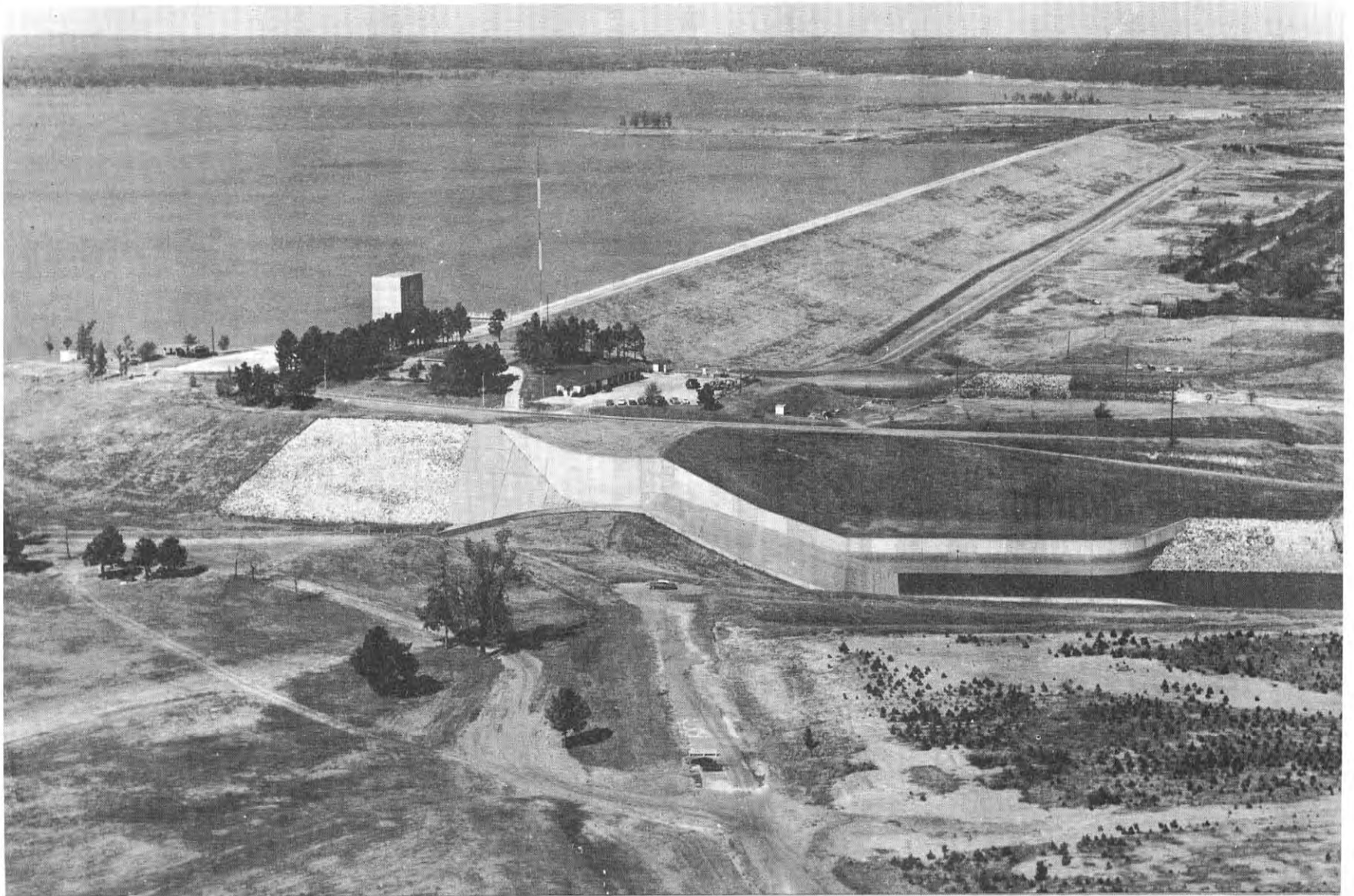
Texarkana Dam and Texarkana Reservoir. Furnished by U. S. Army Corps of Engineers, New Orleans District.
