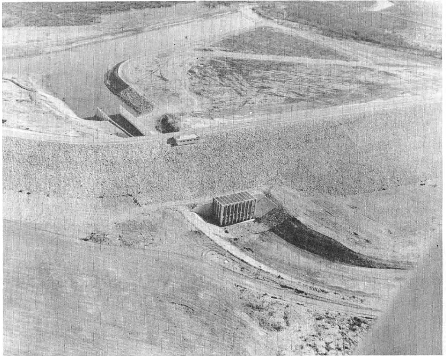
Twin Buttes Dam and Twin Buttes Reservoir. Furnished by U. S. Bureau of Reclamation, Austin Development Office.
