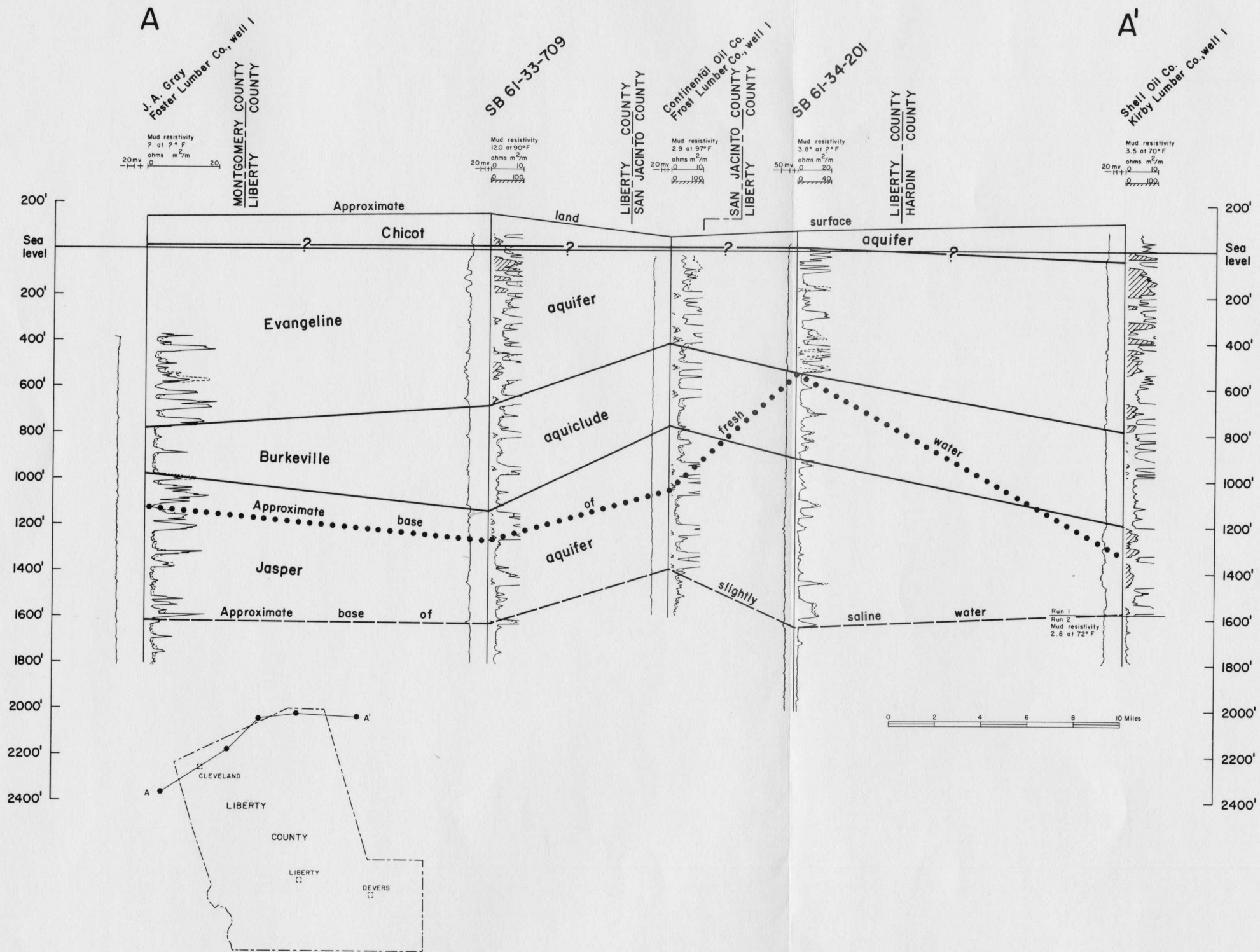
Figure 18 Section A-A' Showing Hydrologic Units and the Approximate Bases of Fresh Water and Slightly Saline Water in Northern Liberty County and Adjacent Areas
