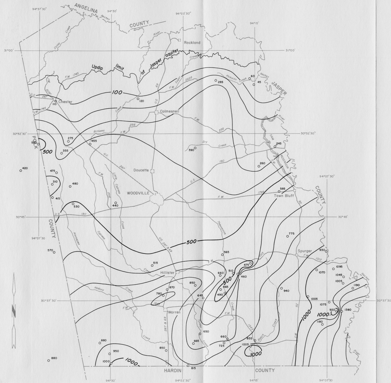
Figure 7 Thickness of Sand Containing Fresh to Slightly Saline Water in the Jasper, Evangeline, and Chicot Aquifers
