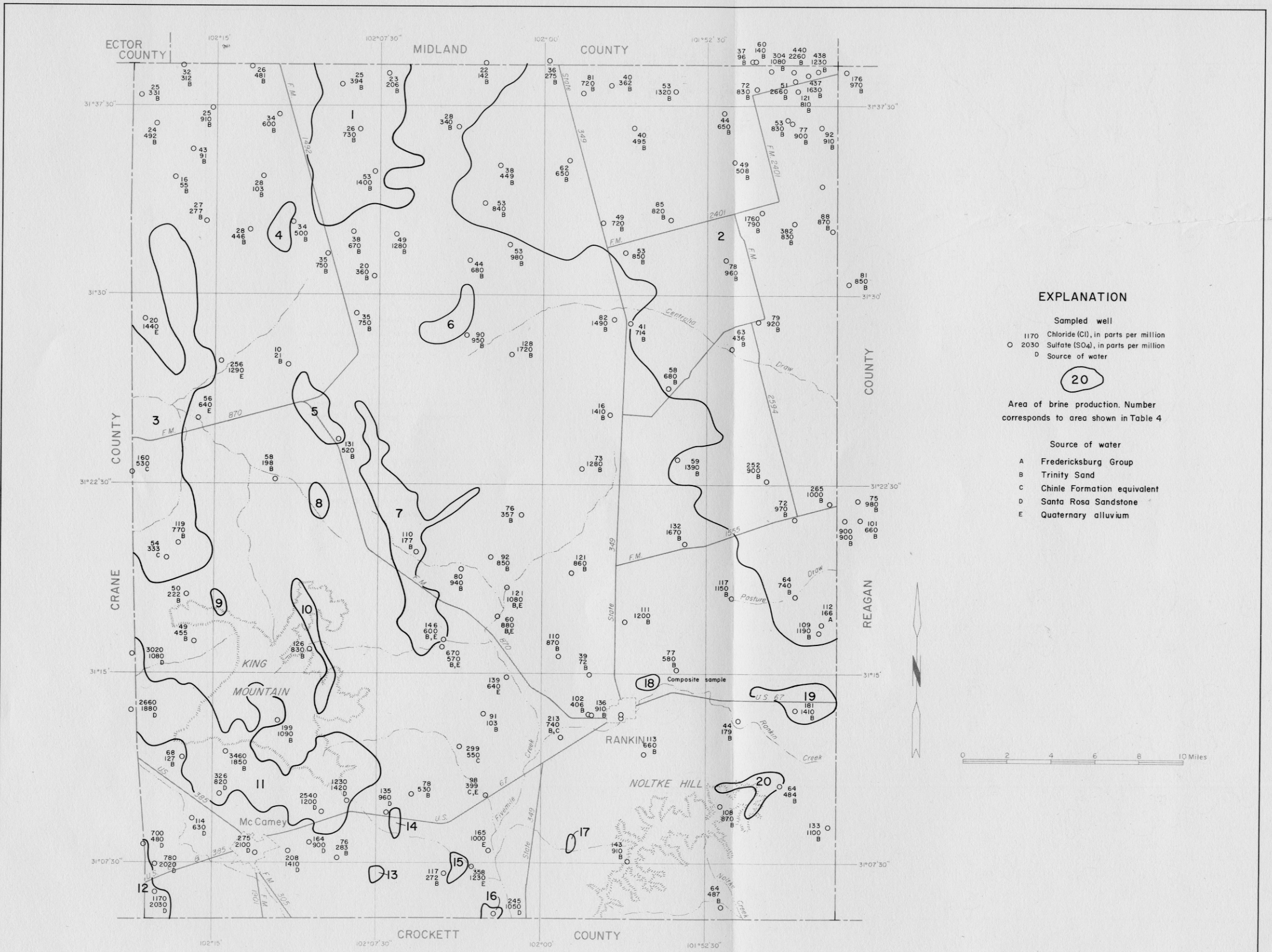
Figure 16 Location of Brine Producing Areas in 1961, and the Chloride and Sulfate Contents of Water From Selected Wells
